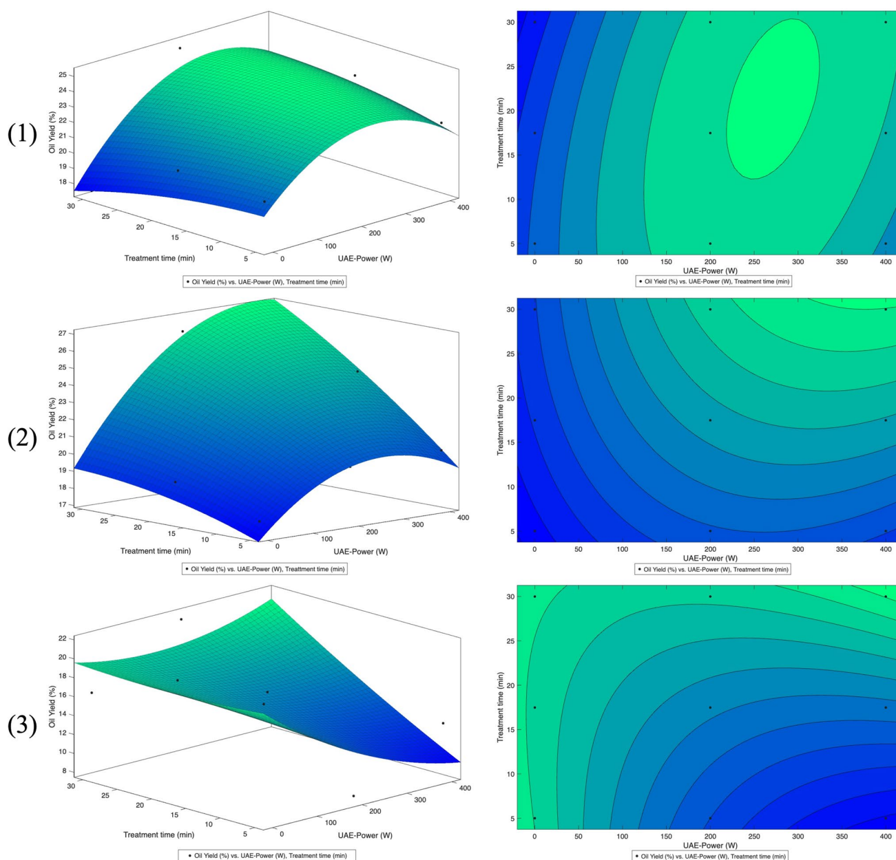
Fig. 4 Response surface (left) and contour (right) plots illustrating the combined effects of ultrasound power (W) and treatment time (min) on extraction yield (%) under three solvent systems: (1) pure
