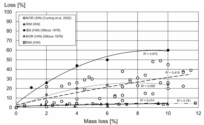
Fig. 7 Relationship between loss of various mechanical properties ( IBS – impact bending strength; MOR – modulus of rupture; RIM – resistance to impact milling) and mass loss of wood due to early decay by white-rot fungi in case of softwoods (SW) and hardwoods (HW). Results were taken from Wilcox (1978) ( IBS , MOR (HW) and Curling et al. (2002b) ( MOR (SW)
