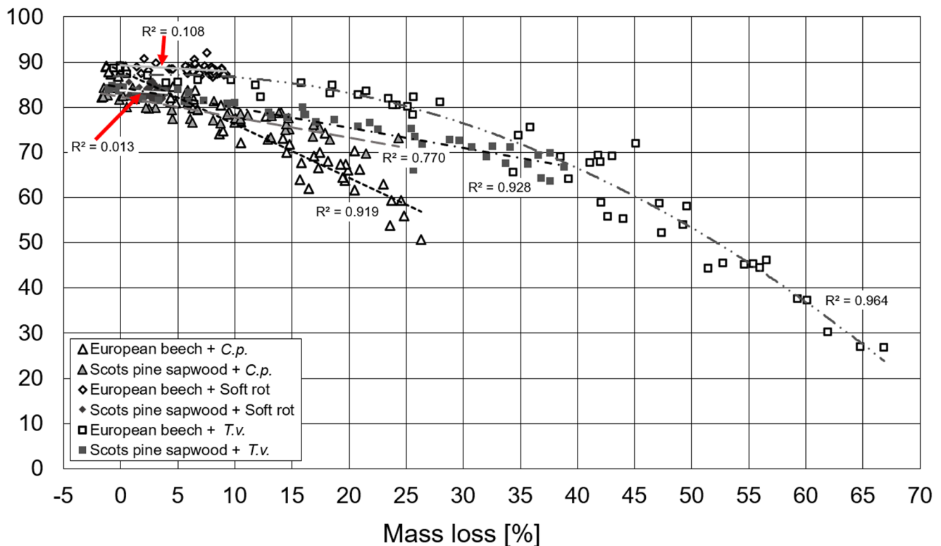
Fig. 3 Resistance to impact milling RIM [%] of Scots pine ( Pinus sylvestris ) sw and European beech ( Fagus sylvatica ) vs. mass loss [%], caused by Coniophora puteana ( C.p. ), soft-rot fungi, or Trametes ver-
