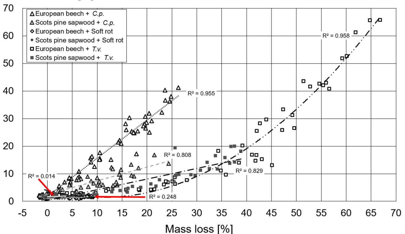
Fig. 5 Fine fraction F [%] of Scots pine ( Pinus sylvestris ) sw and European beech ( Fagus sylvatica ) vs. mass loss [%], caused by Coniophora puteana ( C.p. ), soft-rot fungi, or Trametes versicolor ( T.v. ). Each data
