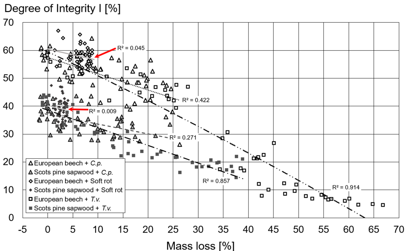
Fig. 4 Degree of integrity I [%] of Scots pine ( Pinus sylvestris ) sw and European beech ( Fagus sylvatica ) vs. mass loss [%], caused by Coniophora puteana ( C.p. ), soft-rot fungi, or Trametes versicolor
