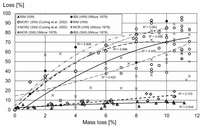
Fig. 6 Relationship between loss of various mechanical properties ( IBS – impact bending strength; MOR – modulus of rupture; RIM – resistance to impact milling) and mass loss of wood due to early decay by brown-rot fungi in case of softwoods (SW) and hardwoods (HW). Results were taken from Wilcox (1978) ( IBS , MOR ) and Curling et al. (2002b) ( MOR1 - Gloeophyllum trabeum ; MOR2 - Postia placenta )
