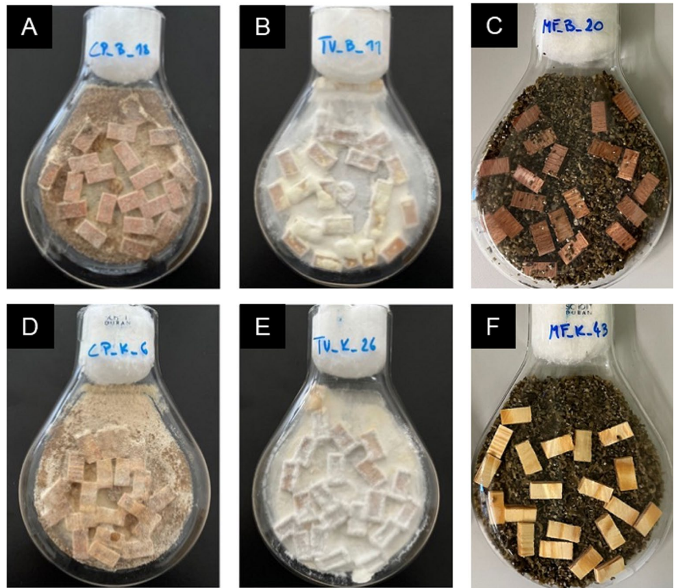
Fig. 1 Kolle flasks containing wood specimens (20 per flask) with dimensions of 10 mm (axial) × 5 mm × 20 mm during incubation. (A) C. puteana on European beech, (B) T. versicolor on European beech, (C) Soft-rot fungi on European beech, (D) C. puteana on Scots pine sw, (E) T. versicolor on Scots pine sw, (F) Soft-rot fungi on Scots pine sw. One replicate sample consisted of 20 single specimens
