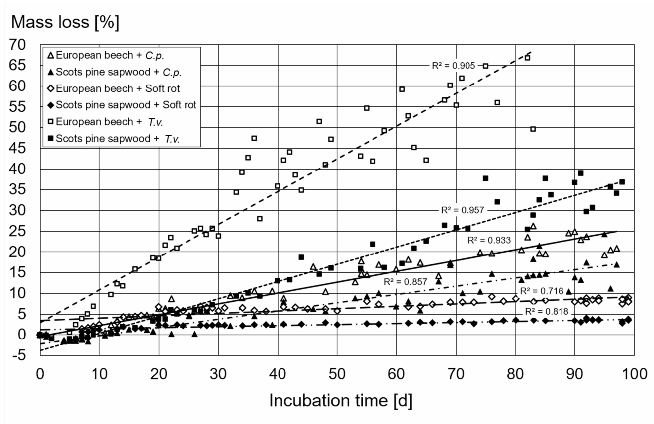
Fig. 2 Mass loss [%] of Scots pine ( Pinus sylvestris ) sw and European beech ( Fagus sylvatica ) over incubation time [days], caused by Coniophora puteana ( C.p. ), soft-rot fungi, or Trametes versicolor
