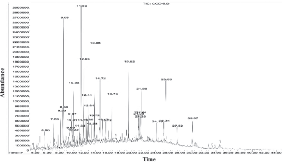
Figure 2. GC-MS chromatogram of L. shawii stem essential oil.
