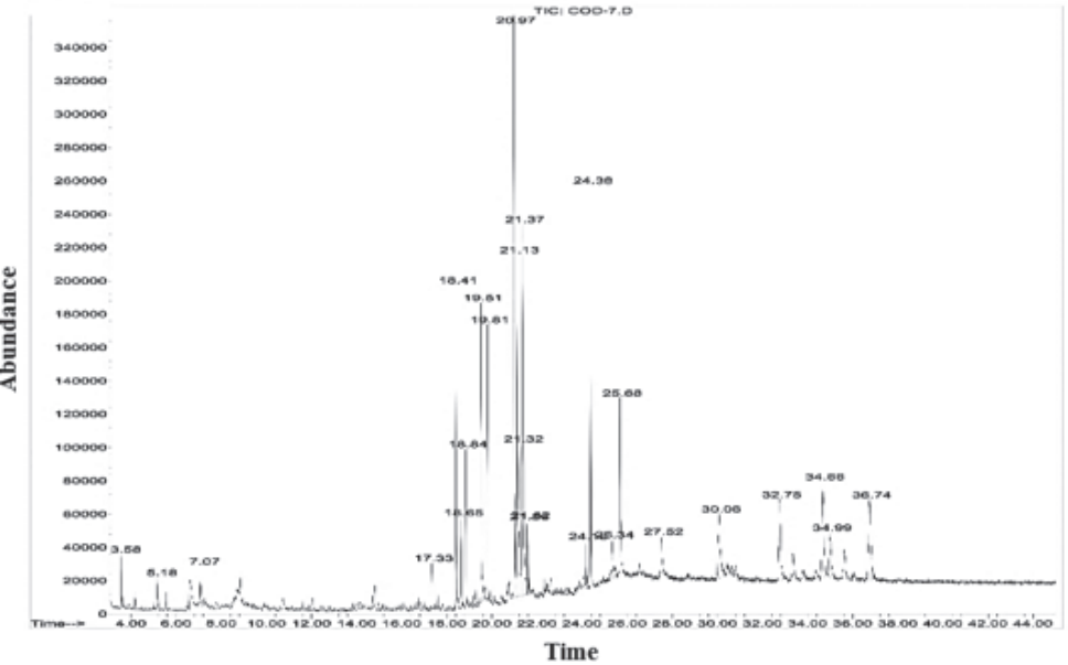
Figure 3. GC-MS chromatogram of L. shawii leaf extract.
