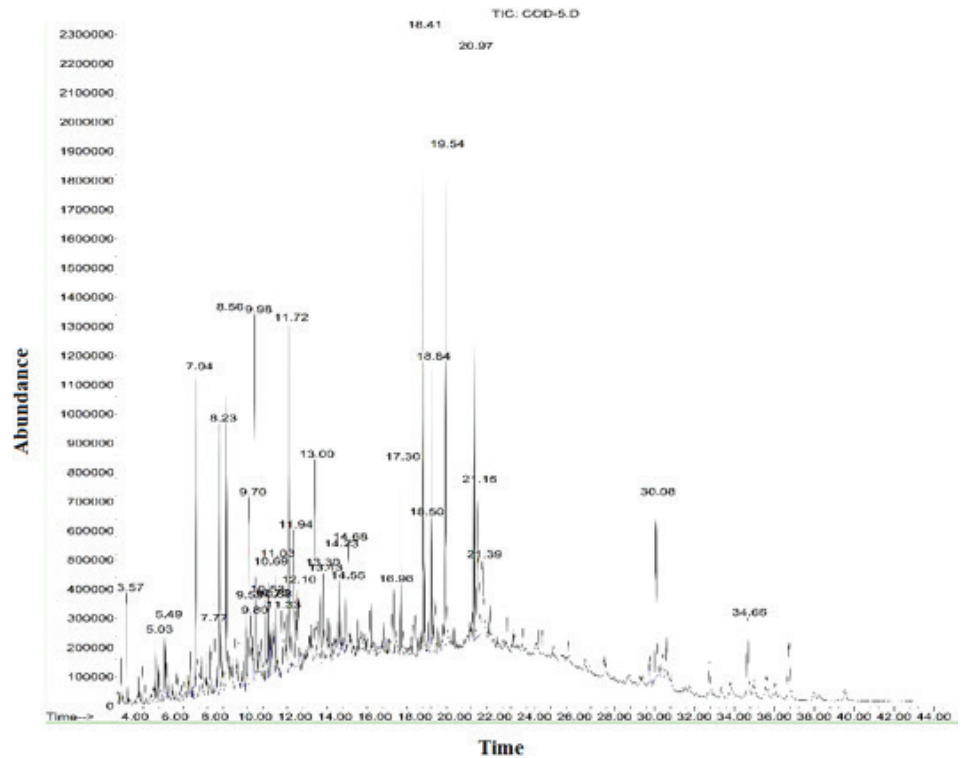
Figure 1. GC-MS chromatogram of L. shawii leaf essential oil.
