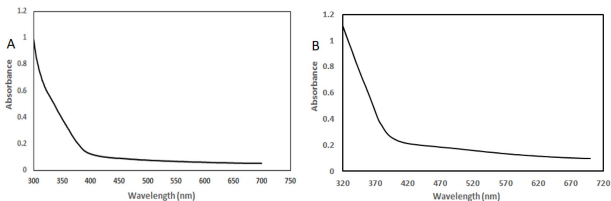
Fig. 1 UV-visible spectrum of the AgNPs synthesized from C. medica fruit extract. A Met-AgNPs. B Eth-AgNPs
