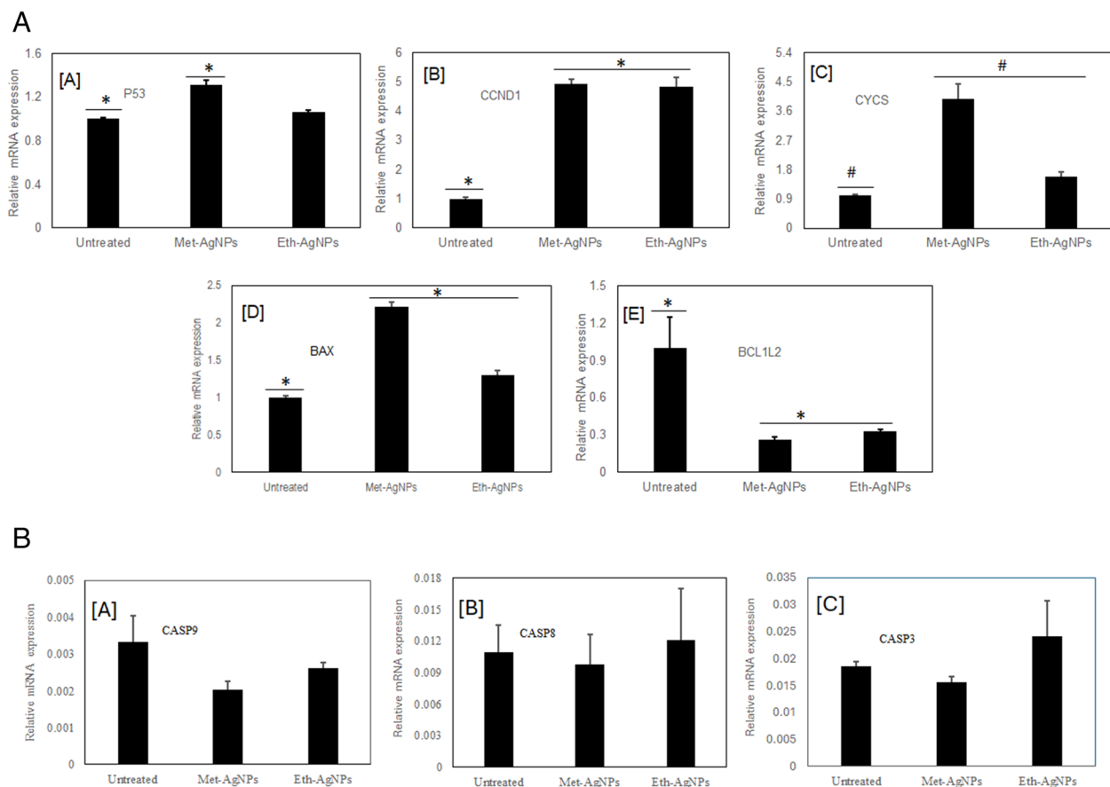
Fig. 10 A Relative mRNA expression of genes of MCF-7 cancer cell lines treated with either Met-AgNPs or Eth-AgNPs. A TP53 gene expression, p -value between untreated vs. Meth-AgNPs < 0.05 . B CCND1 gene expression, p -value untreated vs. Met-AgNPs < 0.05 ; untreated vs. Eth-AgNPs < 0.05 . C CYCS gene expression, p -value untreated vs. Met-AgNPs < 0.05 , untreated vs. Eth-AgNPs < 0.05 . D and E BAX gene expression, p -value between untreated vs. Met-AgNPs < 0.05 and untreated vs. Eth-AgNPs < 0.05 . E BCL2L1 gene expression, p -values untreated vs. Met-AgNPs < 0.05 , untreated vs. Eth-AgNPs < 0.05 . B Relative mRNA expression of genes CASP9 ( A ), CASP8 ( B ), and CASP3 ( C ) of the MCF-7 cells treated with either Met-AgNPs or Eth-AgNPs. The p -values are statistically not significant between groups
