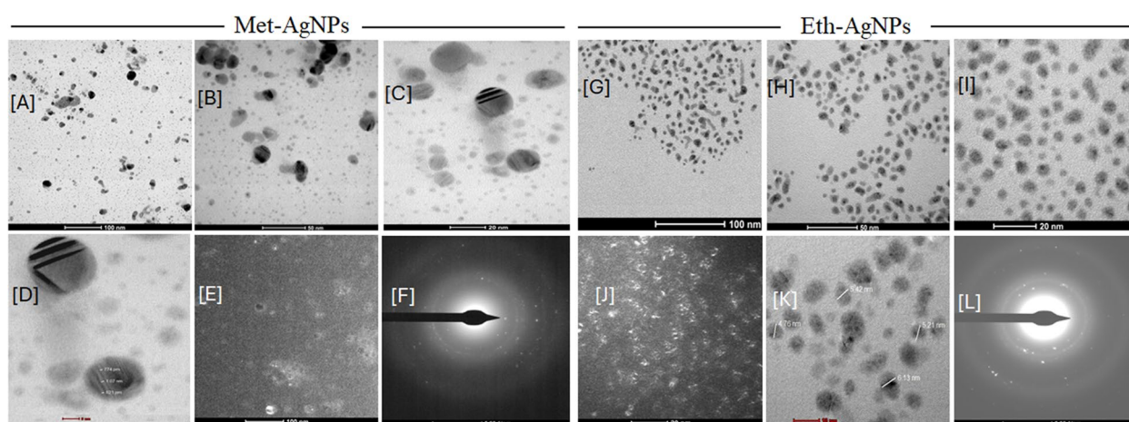
Fig. 5 TEM images of Met-AgNPs (A, B, C, D, E, F) with varying magnifications (A, B, C). Dark-field image (D), HR-TEM image with fringes (E), and SAED image of AgNPs (F). TEM images of Eth-AgNPs (G, H, I, J, K, L) with varying magnifications (G, H, I). Dark-field image (J). HR-TEM image with fringes (K) and SAED image of AgNPs (L)
