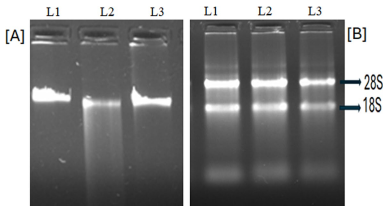
Fig. 9 DNA fragmentation study of the MCF cells treated with L1-Control, L2-Eth-AgNPs, and L3-Met-AgNPs (A). The image of RNA extracted from the MCF-7 cells treated with AgNPs on 1.2% agarose gel, L1-Control, L2-Eth-AgNPs, and L3-Met-AgNPs (B)
