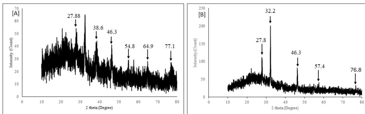
Fig. 4 XRD spectrum of the biosynthesized AgNPs. A Met-AgNPs. B Eth-AgNPs
