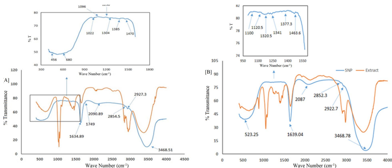
Fig. 2 FTIR spectrum of biosynthesized AgNPs. A Methanolic extract and Met-AgNPs. B Ethanolic extract and Eth-AgNPs
