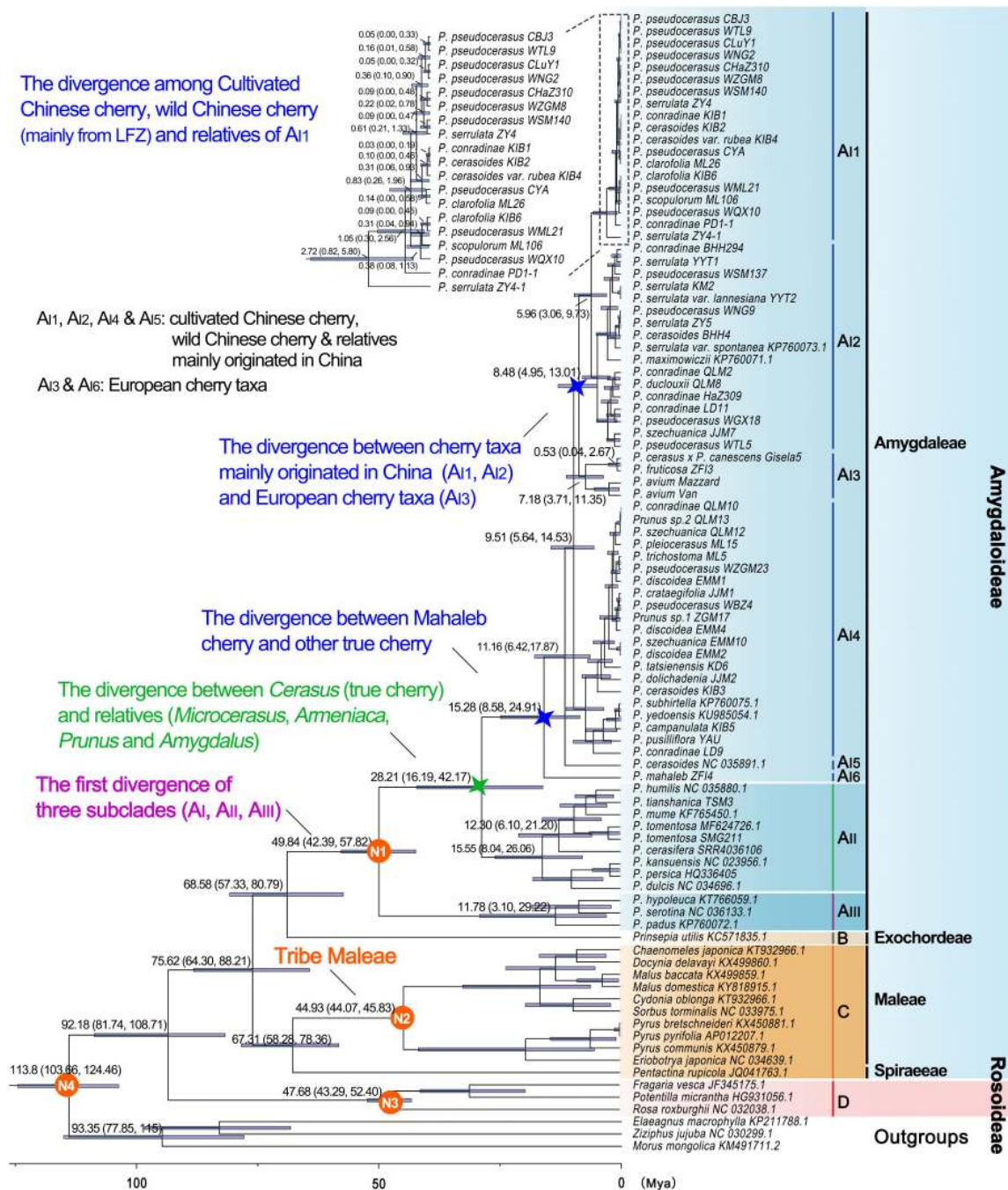
FIGURE 4 | Divergence times of Rosaceae crops based on pruned PWGD. Position of the calibration points N1, N2, N3, and N4 were marked within the tree. Median values and 95% highest posterior density (HPD) were shown next to major branches. The clades A1–A16, AII, AIII, B, C, and D correspond to those in Figure 3 . The divergence between Cerasus (true cherry) and other relatives ( Microcerasus , Armeniaca , Amygdalus , and Prunus ) was marked with green star, and the divergence between European cherry taxa ( Prunus mahaleb , Prunus avium , Prunus fruticosa , and Prunus cerasus × Prunus canescens ) and other true cherries were marked with blue stars.
