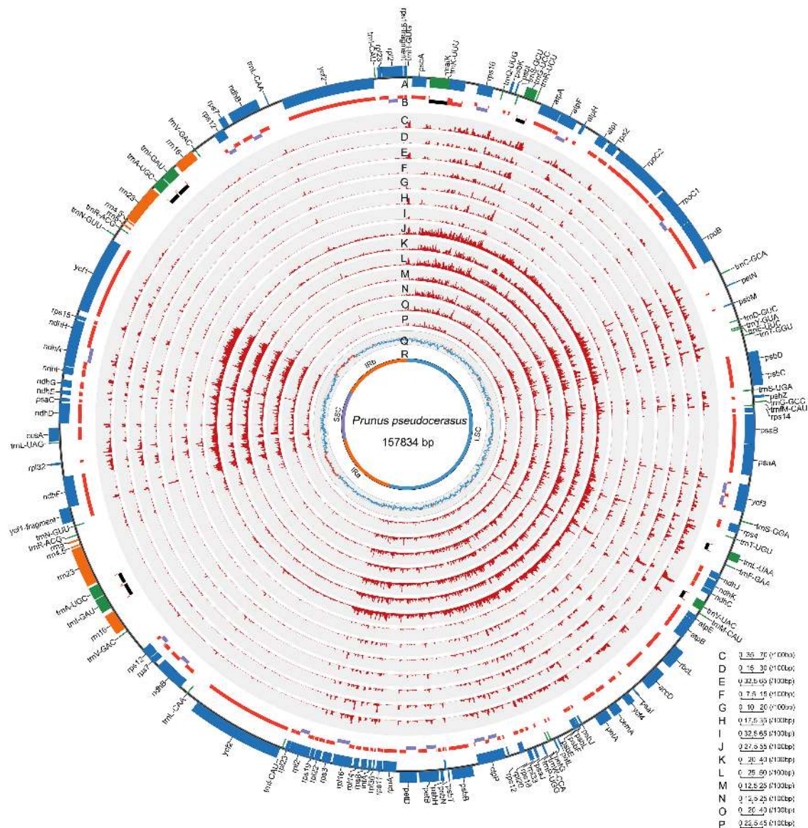
FIGURE 1 | Landscape of genomic variations across the 121 Rosaceae plastomes. A. Gene distribution (blue, protein-coding genes; green, tRNAs; orange, rRNAs). B. Exons and introns (red, exons in protein-coding genes; black, exons in tRNAs; purple, introns). C-I/J-P. Density of insertion-deletion (InDel)/single nucleotide polymorphism (SNP) in plastomes of the Rosaceae family, Rosoideae and Amygdaloideae subfamilies, and Spiraeaceae, Exochordeae, Maleae, and Amygdaleae tribes (100-bp window). Q/R. GC contents/distributions of large single-copy (LSC), short single-copy (SSC) and two inverted repeats (IRs) (100-bp window; light blue, GC content over 50%; orange, GC content below 50%). Prunus pseudocerasus ( Cerasus pseudocerasus ) (NC030599.1) was used as reference genome.
