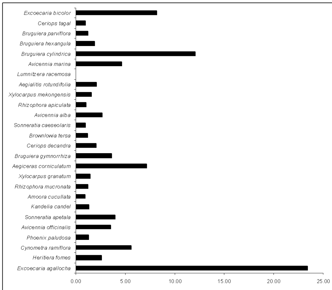
Fig. 2. Population density (No. /100m 2 ) of selected mangrove trees in Lothian Wild Life Sanctuary (Note: Out of 34 true mangrove species, population count was done only for 26 species as per the criterion for carbon assessment DBH \geq 5 cm)
