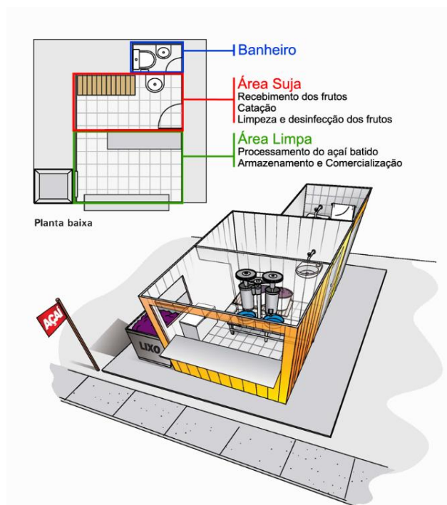
Figure 4 – Layout plan of a suitable açaí processing unit.
