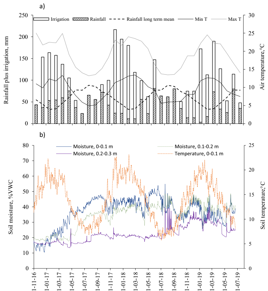
Fig. 1 Environmental parameters at the Allansford site from November 2016 to June 2019: a Monthly precipitation, and irrigation (mm), and maximum and minimum air temperature ( ^{\circ}\text{C} ) plus long-term (25 years) rainfall; b Daily soil volumetric moisture (0–0.1 m, 0.1–0.2 m and 0.2–0.3 m) and soil temperature (0–0.1 m)
