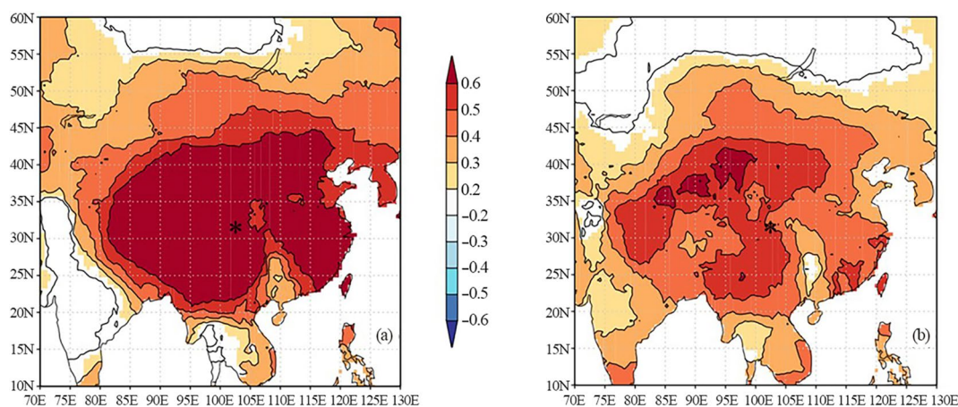
Fig. 8 Spatial correlations of the a actual and b reconstructed T_{6-11} with CRU TS4.03 temperatures during 1961–2016. The star denotes the sampling site
