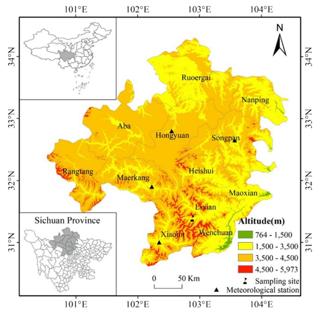
Fig. 1 Location of the study site (flag) and nearby meteorological stations (triangles)
