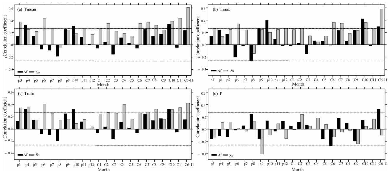
Fig. 4 Correlations between climate factors (Tmean, Tmax, Tmin, P) and chronologies of A. faxoniana (Af) and S. saltuaria (Ss) during 1961–2016. Months of p3–p12 indicate previous March to previous December; Months of C1–C11 indicate current January to current
