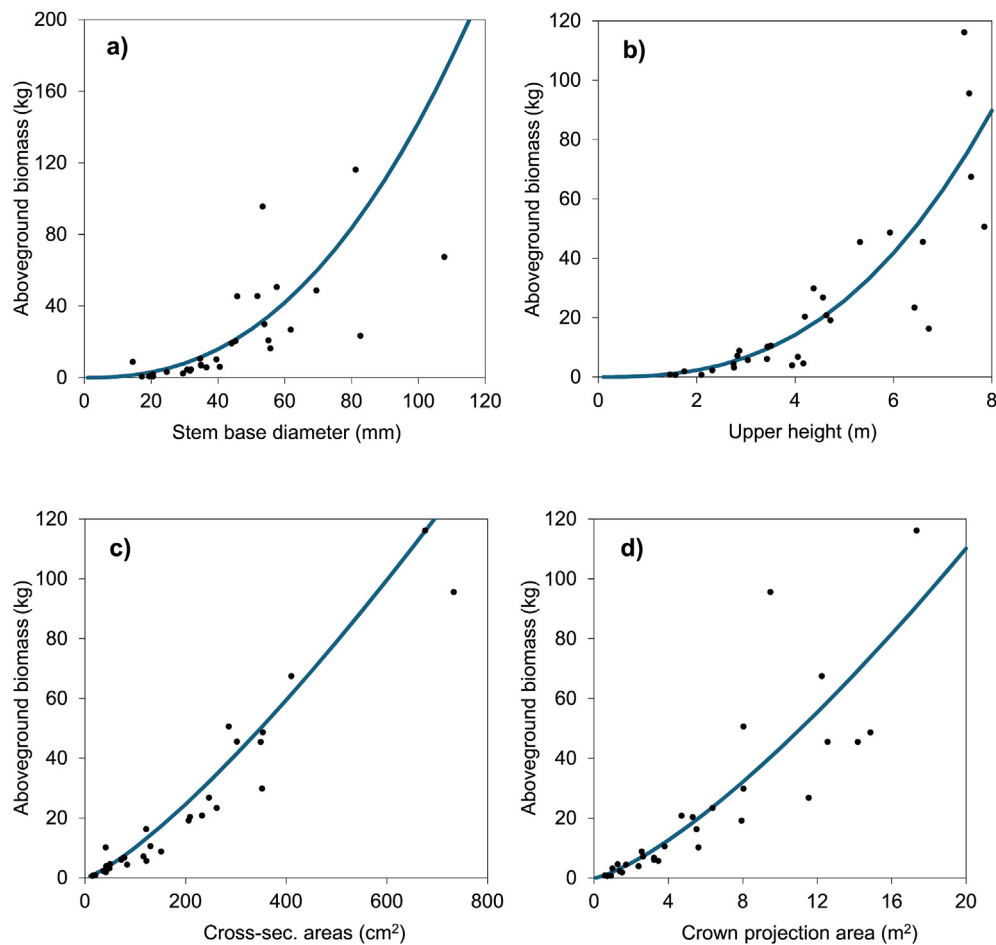
Fig. 2. Model fits predicting aboveground biomass (lines) as a function of the stem base diameter of the thickest stem (a), maximum height (b), the sum of cross-sectional areas of all stems at base (c), and crown projection area (d) of a single European hazel shrub. Dots represent measured values in 30 individual shrubs.
