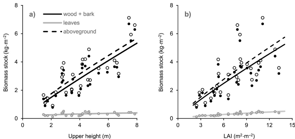
Fig. 3. The relationship between aboveground biomass stock per unit area and its components in European hazel, and shrub height (a) and leaf area index (b). Dots represent measured values, while lines indicate linear model fits.
