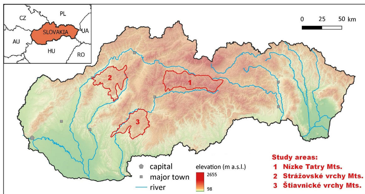
Fig. 1. Location of the study areas for research of aboveground European hazel biomass, Inner Western Carpathians, Slovakia.
