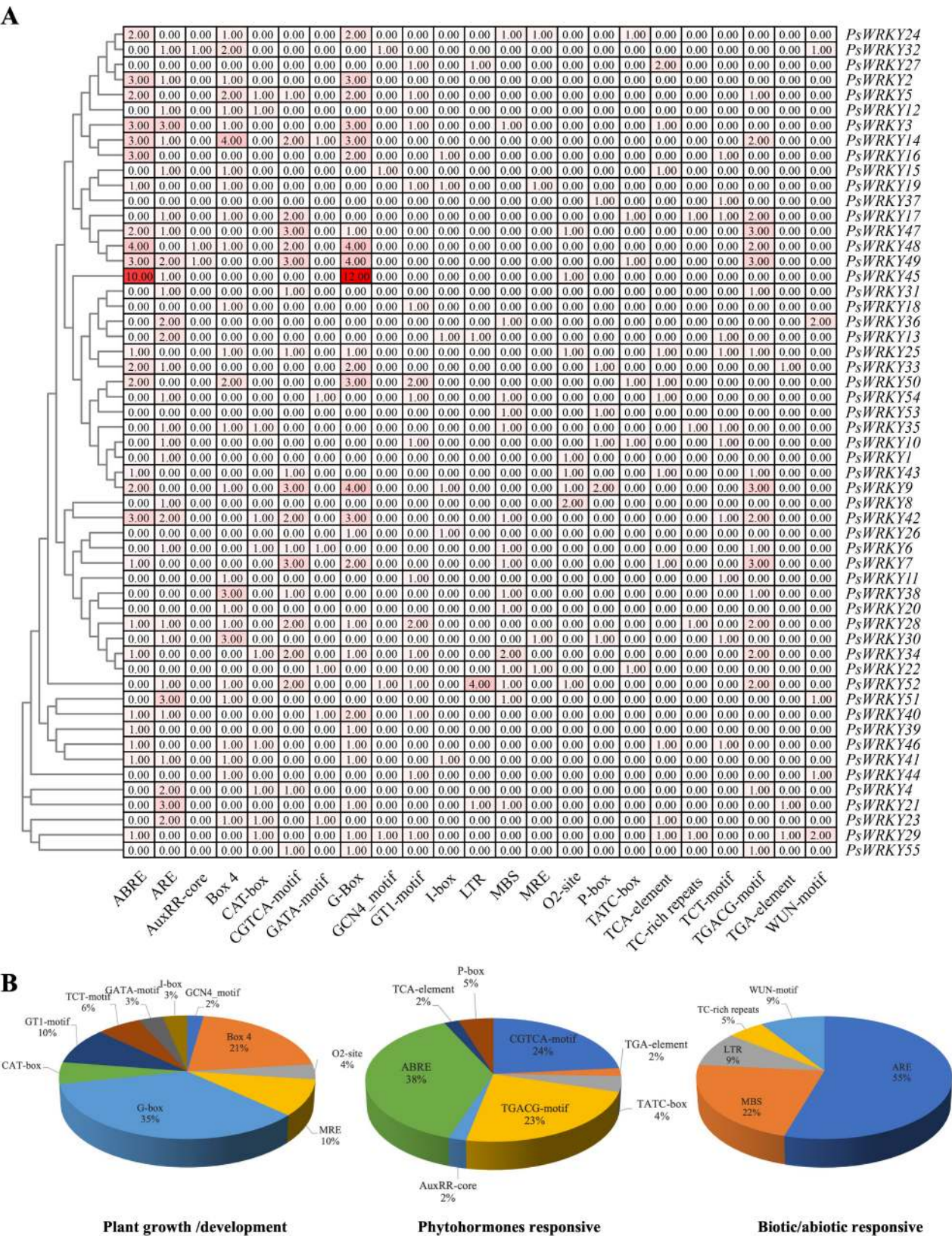
Fig. 7 Analysis of the cis-acting elements of the PsWRKYs .
