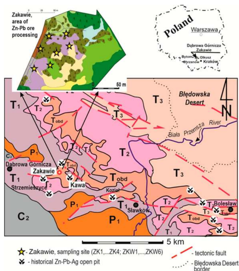
Figure 1. Geological sketch of the study area. Legend: C 2 —UPPER CARBONIFEROUS—USCB boundary, P 1 —Lower Permian, T 1 —Lower Triassic, T 2 —Middle Triassic, T 3 —Upper Triassic, T obd —ore-bearing dolomites with Zn-Pb-Ag mineralization [29].
