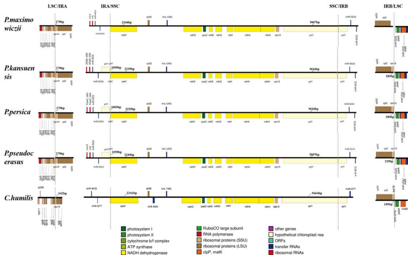
Fig 4. Comparison of the boundaries of the LSC, SSC, and IR regions in the C. humilis chloroplast genome with those of four other Prunus species.
