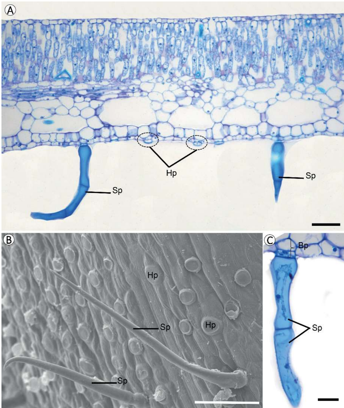
Figure 1. Photomicrographies (A, C) and scanning electron micrograph (B) of Nymphaeaceae leaves. A. Cross section of Victoria amazonica leaf blade showing hydrotypes with sharp-pointed apical portion (Sp) and mature hydrotypes (Hp) in the abaxial surface. B. Abaxial surface of Nymphaea rubra leaf showing hydrotypes with sharp-pointed apical portion (Sp) and mature hydrotypes (Hp). C. Detail of hydrotypic cell with sharp-pointed apical portion in V. amazonica leaf, showing a two-celled apical portion (Ap), and a basal portion (Bp) inserted among the common epidermal cells. Bars: A-B = 100 \mu m, C = 30 \mu m.
