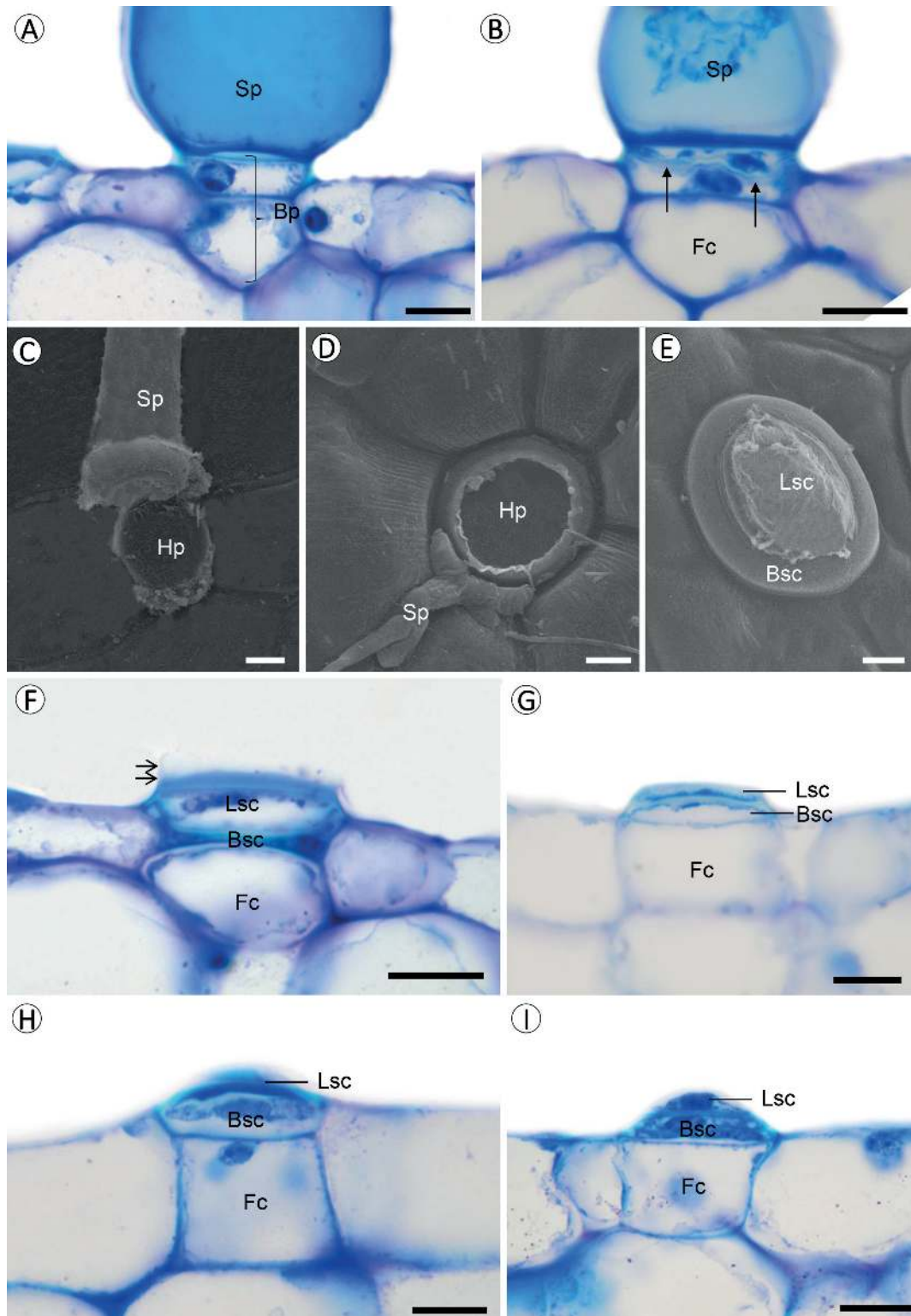
Figure 2. Hydropotes in different developmental stages in Nymphaeaceae species. A,B, F-I. Photomicrographs. C-E. Scanning electron micrographs. A. Hydropote in Victoria amazonica showing a sharp-pointed apical portion (Sp) and a basal portion (Bp) with two short cells. B. The arrows indicate new wall formed by periclinal division of the upper cell in the basal region of the hydropote in V. amazonica . Sp: sharp-pointed apical portion, Fc: Foot cell. C-D. Detachment of the sharp-pointed apical portion (Sp) in hydropote of Nymphaea lotus ( C ) and Nymphaea caerulea ( D ) giving raise to mature hydropotes (Hp). E. Mature hydropote in Nymphaea rubra showing a lens-shaped cell (Lsc) and a bowl-shaped cell (Bsc). F-I. Mature hydropotes showing a large Foot cell (Fc), a bowl-shaped cell (Bsc) and a lens-shaped cell (Lsc) in V. amazonica ( F ), N. lotus ( G ), N. caerulea ( H ) and N. rubra ( I ). Double arrows indicate remaining of the sharp-pointed apical portion. G Bars: A-B, F-I = 15 \mu m, C = 10 \mu m, D-E = 5 \mu m.
