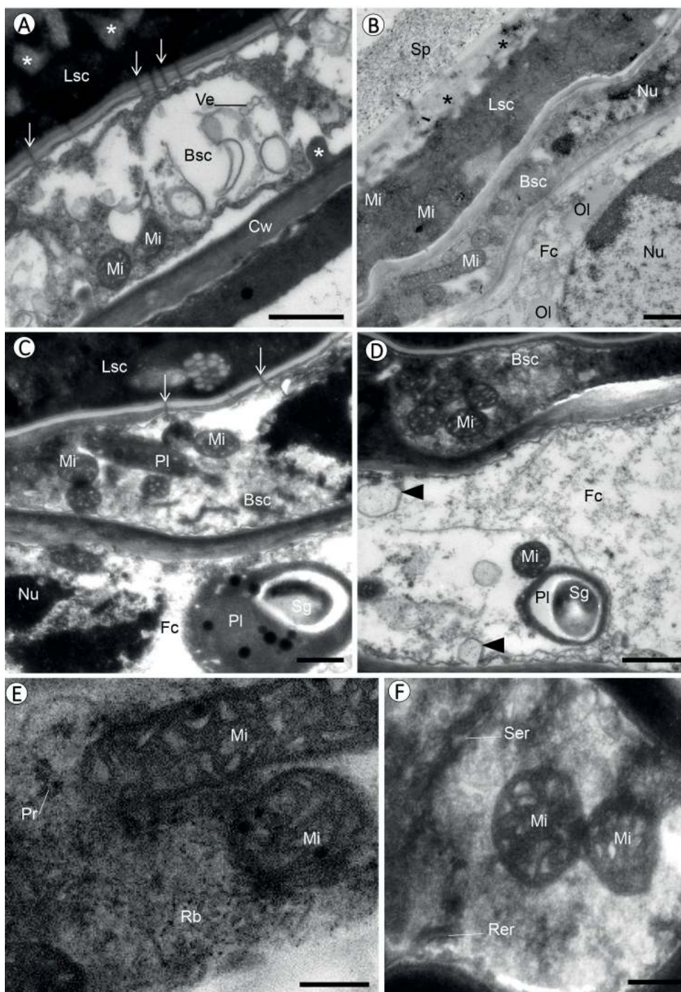
Figure 4. Transmission electron micrographs of the bowl-shaped cell and foot cell of hydropotes in leaves of Victoria amazonica (A) and Nymphaea lotus (B-F). A. Detail of hydropote showing bowl-shaped cell (Bsc) with numerous plasmodesmata (arrows) in the outer periclinal wall and vesicles (Ve) and mitochondria (Mi) in the cytoplasm. Cw: cell wall; *: labyrinthine projections; Lsc: lens-shaped cell. B. Hydropote showing lens-shaped cell (Lsc) with labyrinthine projections (*) in the outer periclinal wall and dense cytoplasm with mitochondria (Mi); bowl-shaped cell (Bsc) with abundant cytoplasm, nucleus (Nu) and mitochondria (Mi) with dilated cristae; foot cell (Fc) with voluminous nucleus (Nu) and oil (Ol) drops in the cytoplasm. Sp: debris of sharp-pointed apical portion. C. Detail showing bowl-shaped cell (Bsc) with plasmodesmata (arrow) connecting it to the lens-shaped cell (Lsc); observe mitochondria (Mi) and plastid (Pl) in the cytoplasm; in the foot cell (Fc) observe plastid (Pl) with plastoglobuli and degrading starch grains (Sg). D. Bowl-shaped cell (Bsc) with abundant mitochondria with dilated cristae, and foot cell (Fc) with electron lucent cytoplasm with mitochondria (Mi), plastids (Pl) with degrading starch grains (Sg), and vesicles (arrowhead) fusing to the plasma membrane. E. Detail of bowl-shaped cell showing cytoplasm with free ribosomes (rb), polyribosomes (Pr) and mitochondria (Mi). F. Bowl-shaped cell with smooth (Ser) and rough (Rer) endoplasmic reticulum and mitochondria (Mi). Bars: A-D = 1 µm, E-F = 0.5 µm.
