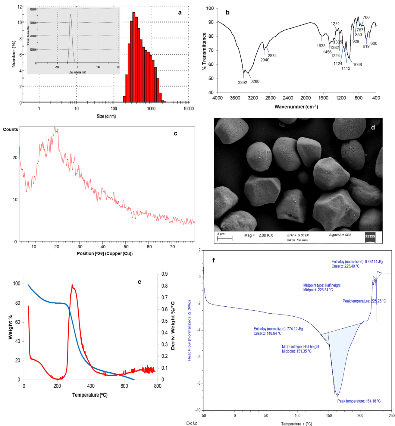
Fig. 5 The DLS and zeta potential (a), FTIR (b), XRD (c), FESEM (d), TGA (e), and DSC (f) of the extracted agar
