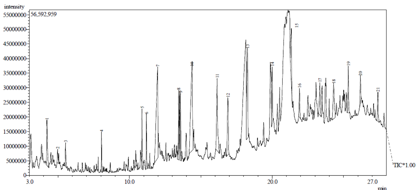
Fig. 2: GC/MS chromatogram of M. sloanei seed hydrocolloids
