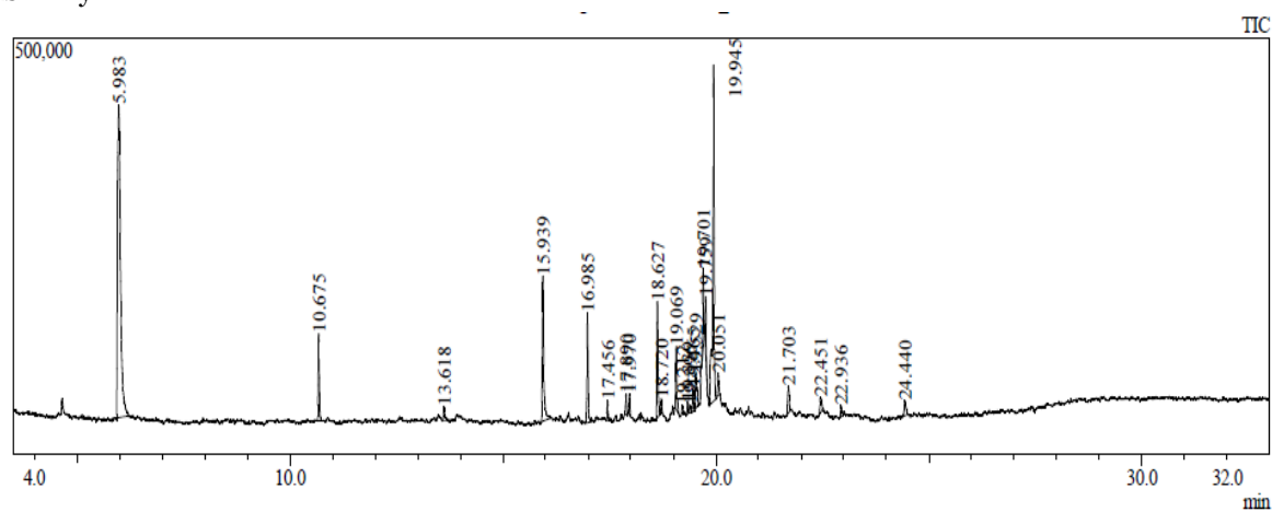
Figure 2: GCMS Analysis of the extract
