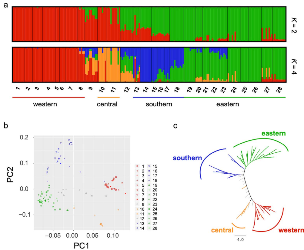
Figure 1. a Population structure of F. nilgerrensis identified with STRUCTURE based on genome-wide SNPs. K=2 shows the highest \Delta K , and K=4 represents the fine-scale structure within F. nilgerrensis . b PCA for all populations based on the same SNP data set as STRUCTURE. (c) Neighbor-joining phylogenetic tree of all samples.
