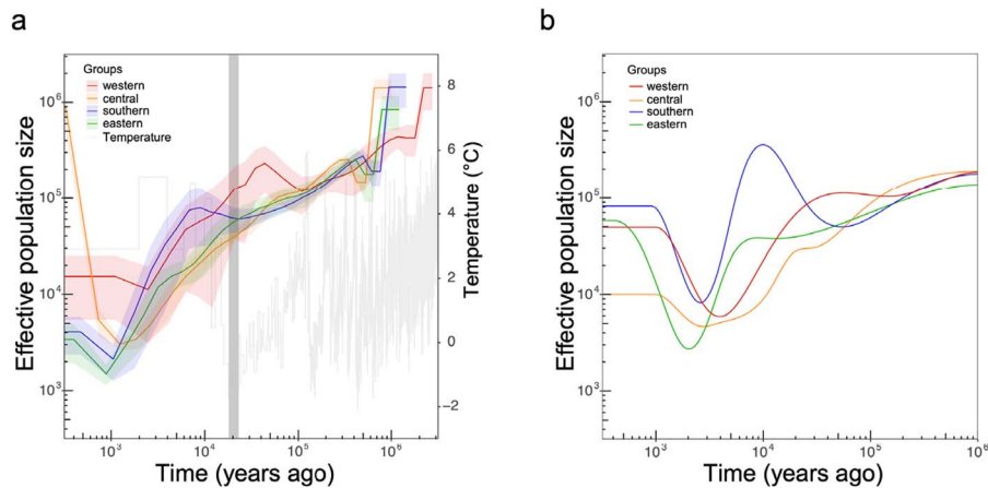
Figure 2. Historical changes in effective population size of the four F. nilgerrensis groups. a Inferred using MSMC based on sets of four haplotypes, with solid lines representing medians and shading representing \pm standard deviation calculated across pairs of haplotypes. The dark gray bar indicates the period of the LGM. b Inferred using SMC++ based on individuals in each group
