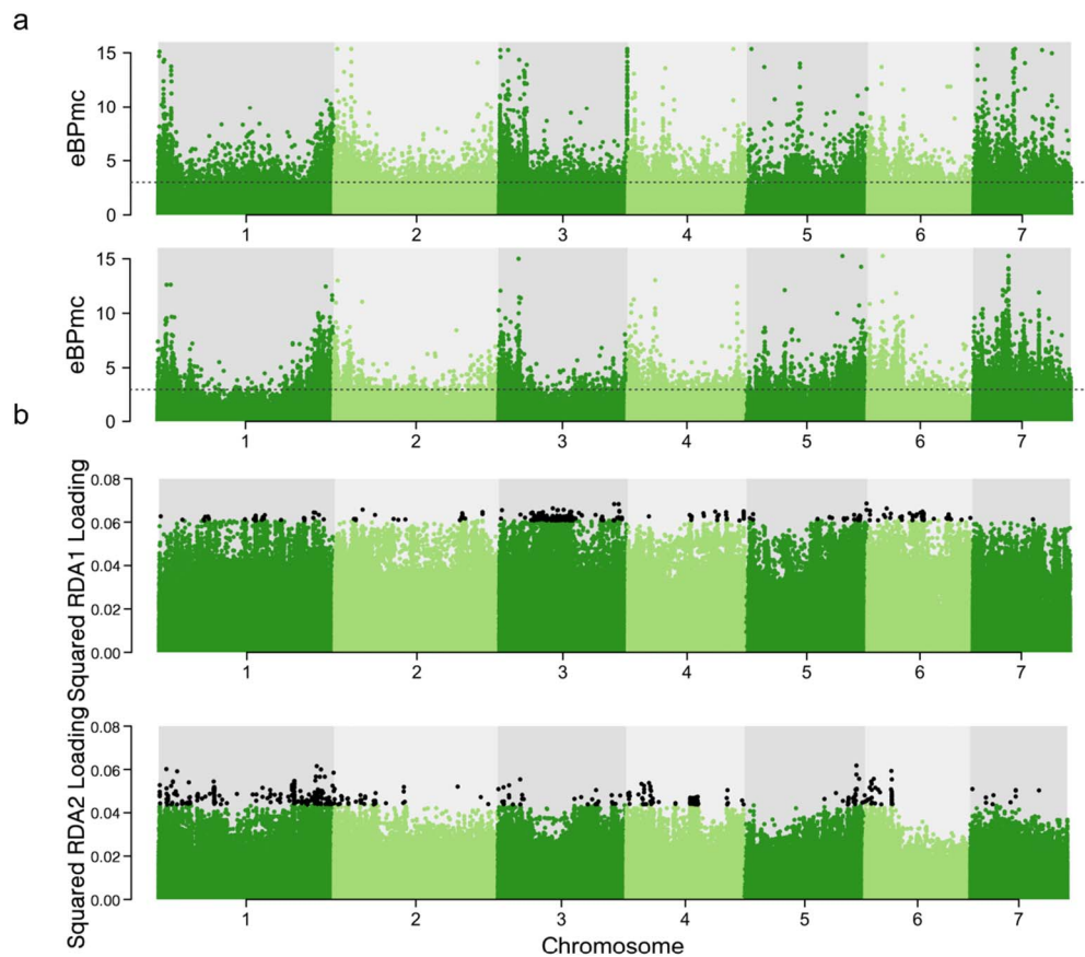
Figure 4. Manhattan plots for the results of GEA. a Empirical Bayesian P-value (eBPmc) for an association with the first environment principal component (top panel) and the second environment principal component (bottom panel). The dotted black line establishes the eBPmc significance threshold at 3. b SNP loadings on the first RDA axis (top panel) and the second RDA axis (bottom panel) accounting for spatial structure among populations. The black dots represent SNPs with significant associations along the RDA axes (at least three standard deviations away from the mean squared loadings). We only show the first two RDA axes here.
