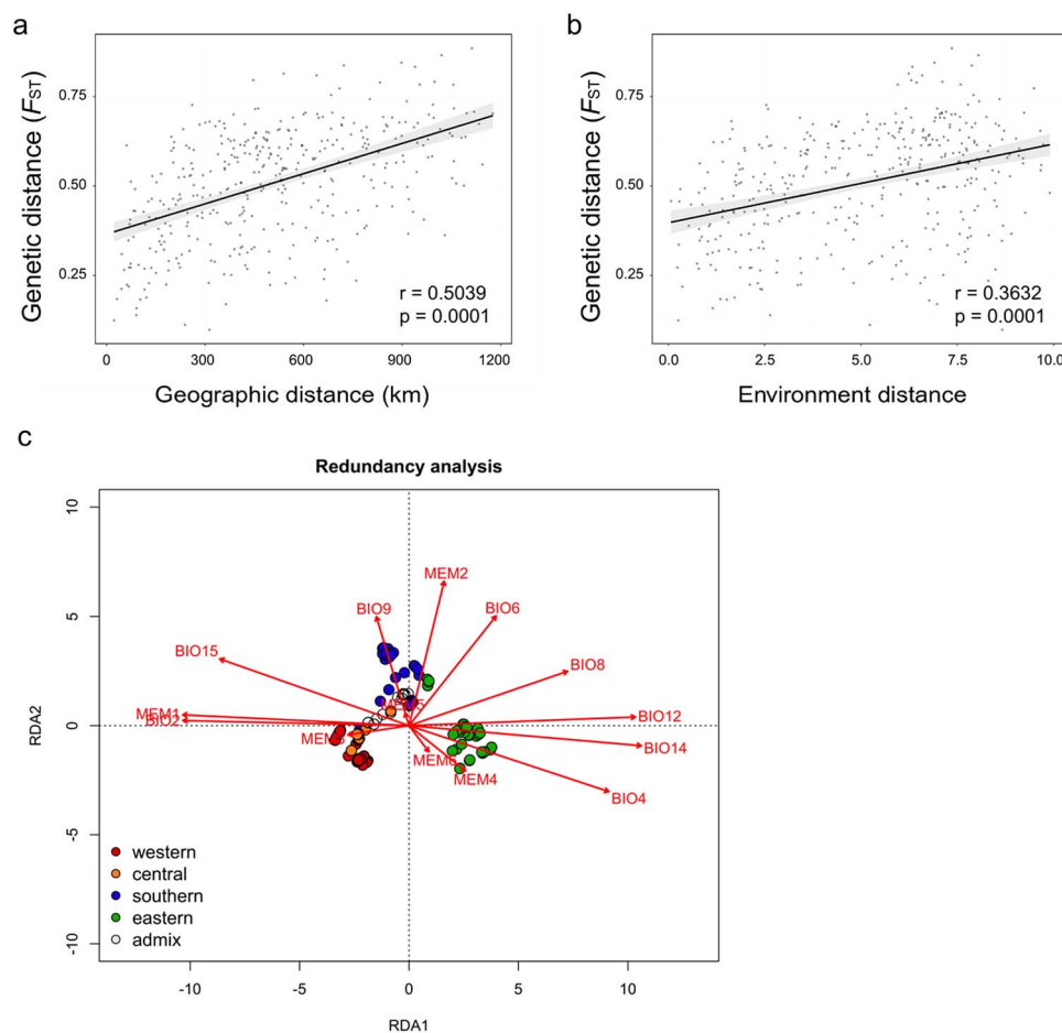
Figure 3. IBD, IBE, and RDA. a Genetic pairwise differentiation plotted against geographic distances. b Environmental distances between populations. c RDA testing the effect of geographic and environmental variables on the degree of genetic differentiation. The first two canonical axes (RDA1 and RDA2) are shown.
