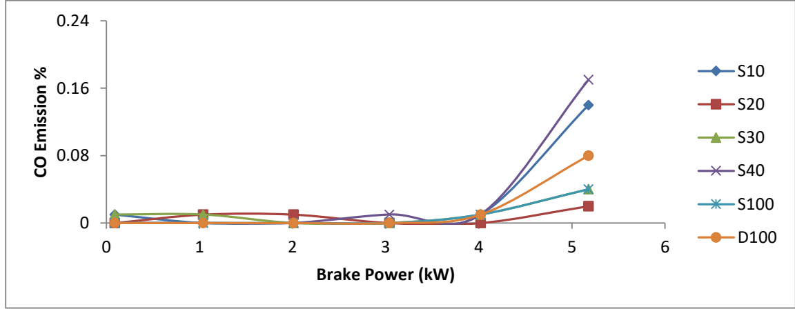
Figure 6. Variation of carbon monoxide with brake power for Simarouba biodiesel blends and diesel.
