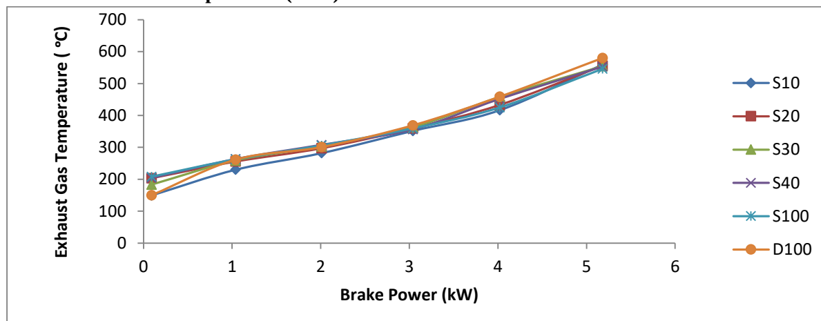
Figure 5. Variation of exhaust gas temperature with brake power for Simarouba blends and diesel.
