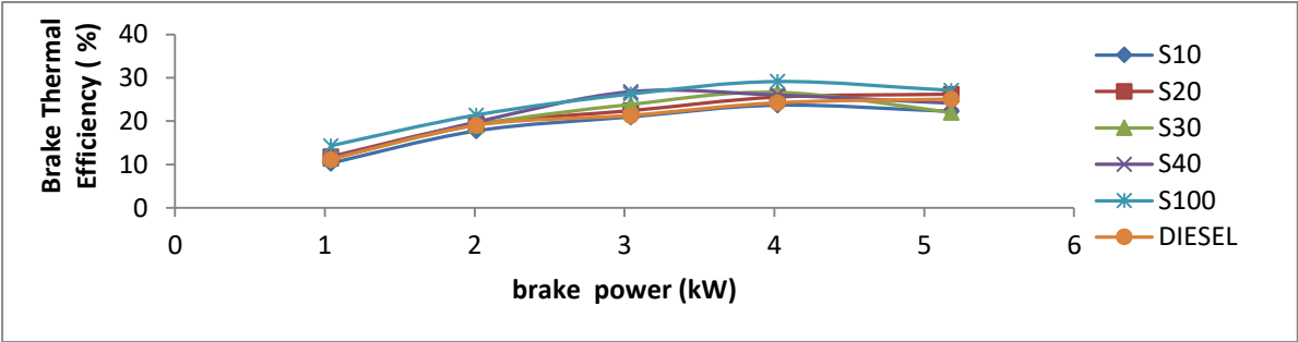
Figure 2. Variation of brake thermal efficiency with brake power for Simarouba blends and diesel.
