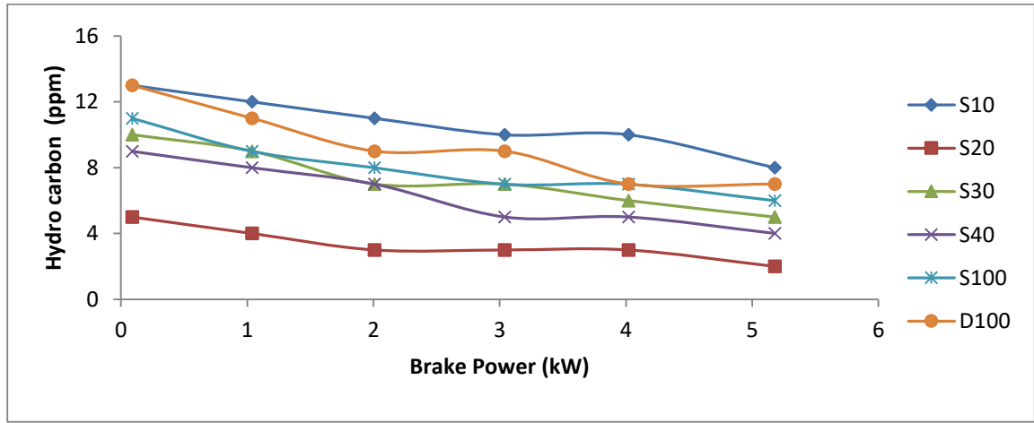
Figure 7. Variation of hydrocarbon with brake power for Simarouba biodiesel blends and diesel.
