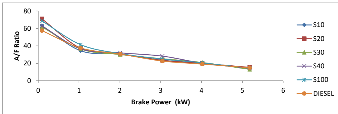
Figure 4. Variation of air fuel ration with brake power for Simarouba biodiesel blends and diesel.
