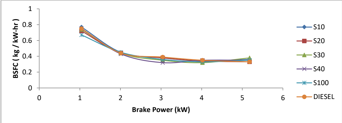
Figure 3. Variation of brake specific fuel consumption with brake power for Simarouba blends and diesel
