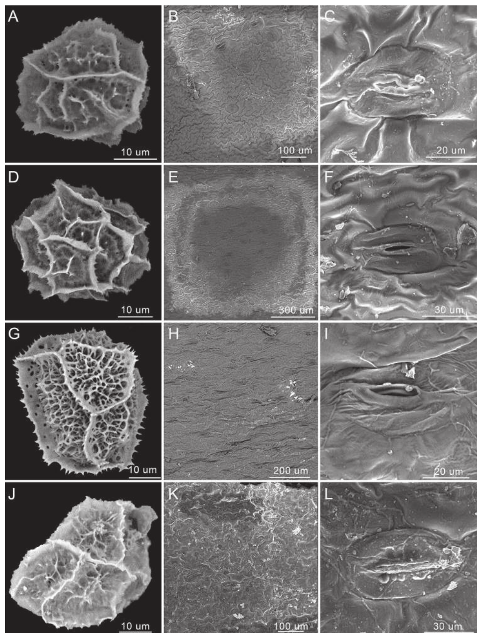
Figure 1. Scanning electron micrographs of spore and stomata of A. alatulum , A. subcrenatum and A. wrightii A–F A. wrightii G–I A. subcrenatum J–L A. alatulum .
