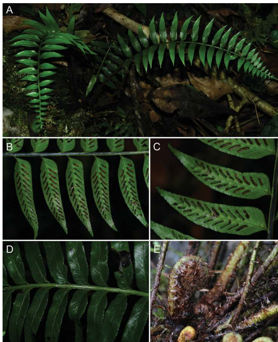
Figure 5. Asplenium subcrenatum A Habitat and habit B Portion of lamina showing abaxial view of pinna C Abaxial view of pinna showing the serrate to coarsely dentate margin D Adaxial view of upper portion of lamina E Lower portion of stipes showing the reddish-brown scales.
