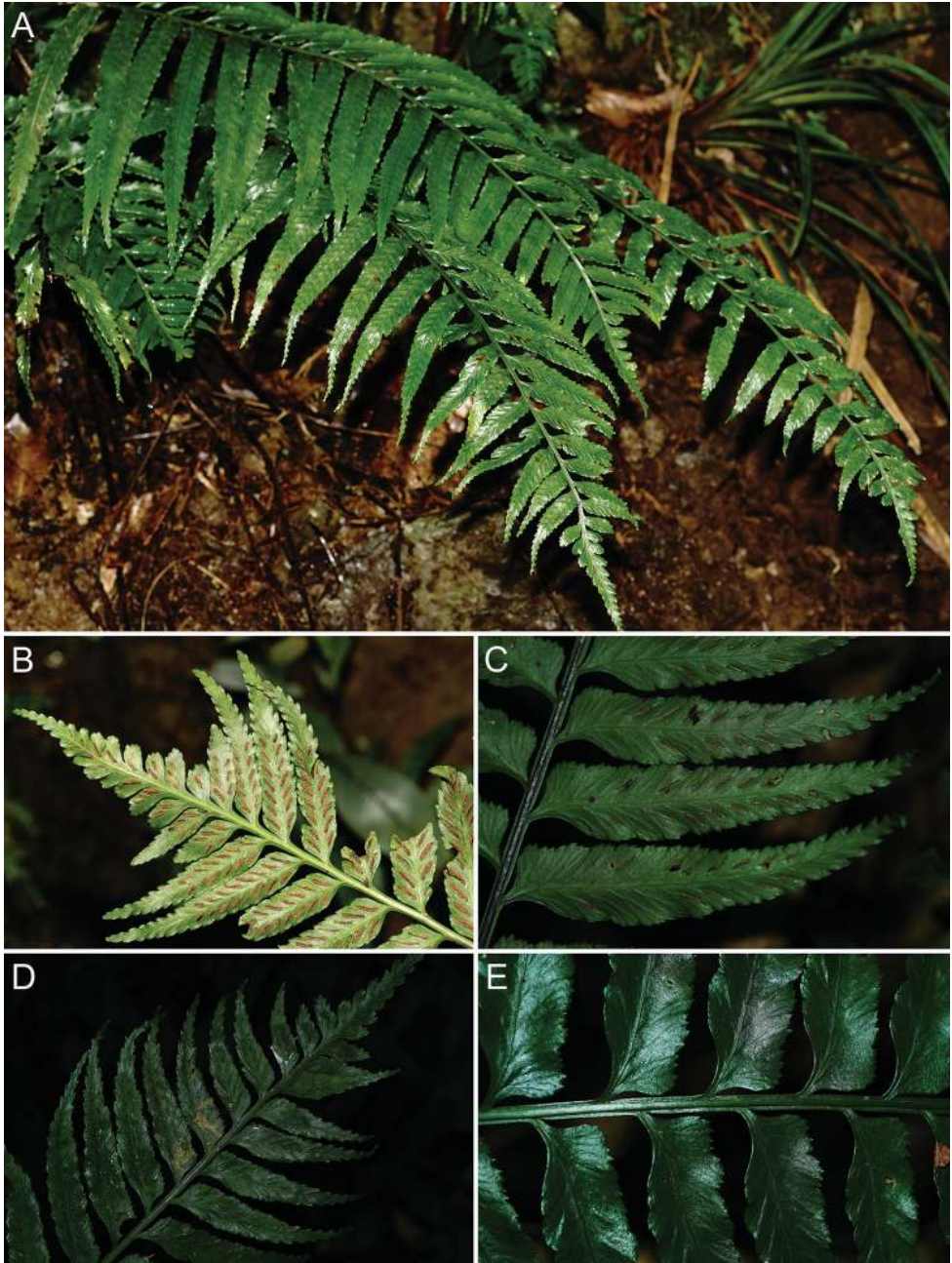
Figure 6. Asplenium wrightii A Habitat and habit B Abaxial view of upper portion of lamina C Abaxial view of pinna showing the almost entire to crenate-sinuate margin D Adaxial view of upper portion of lamina E Upper portion of rachis showing the lateral wings.
