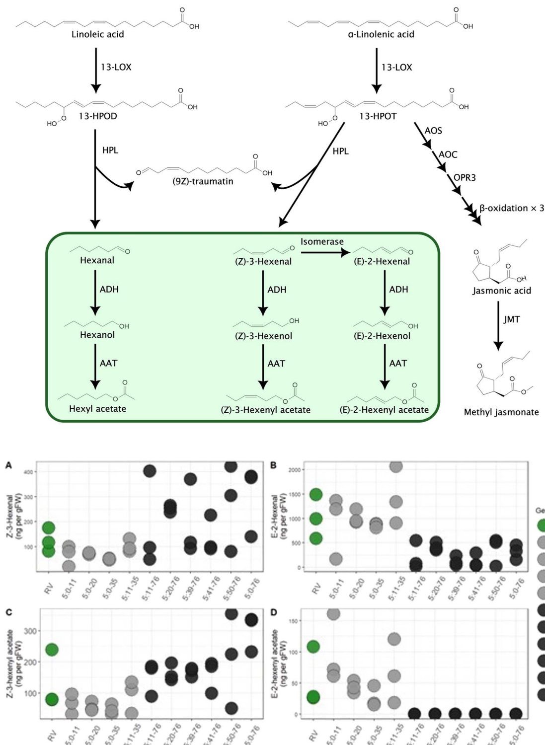
Figure 1. Biosynthetic pathway of Linoleic acid and accumulation of the GLV in strawberry samples A) (Z)-3-hexenal, B) (E)-2-hexenal, C) (Z)-3-hexenyl acetate, and D) (E)-2-hexenyl acetate in RV and LG5 introgression lines, determined as ng/g of fresh weight in red ripe berries. Three biological replicates for all genotypes were independently analysed on the same day they were prepared.
