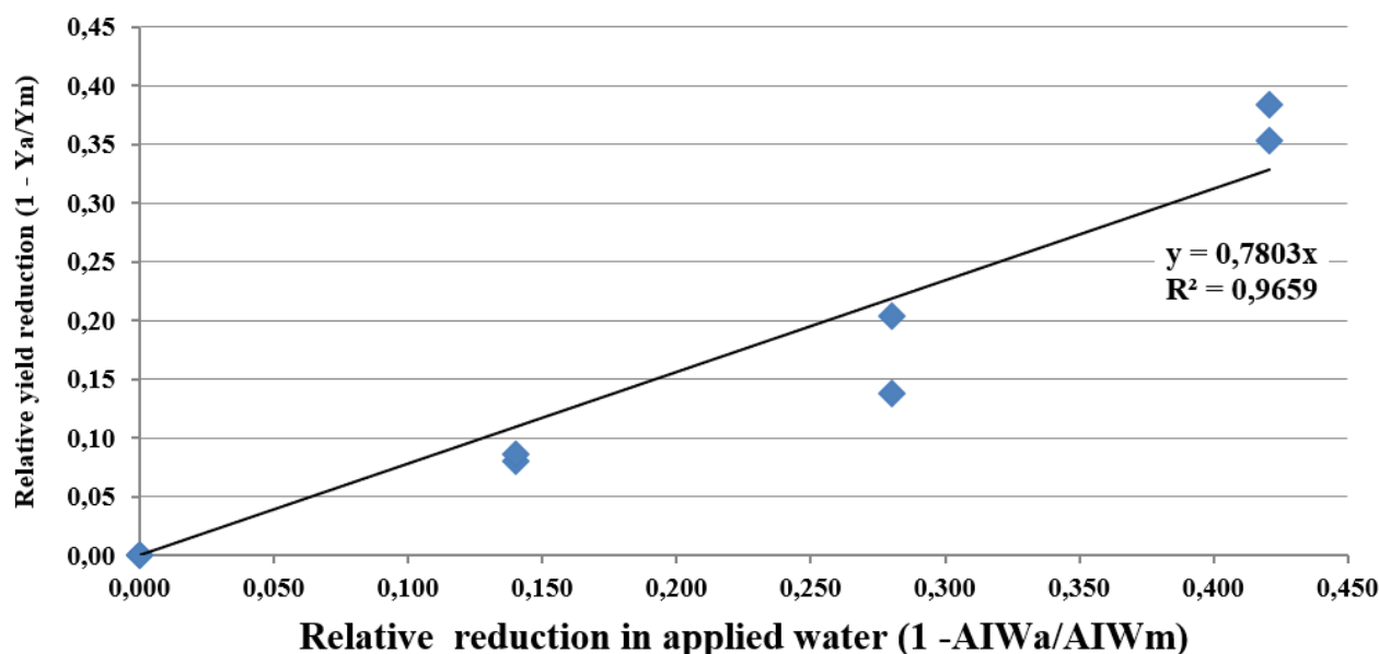
Figure 4: Yield response factor ( K_y ) of chia crop
