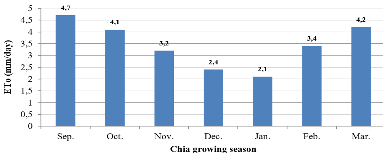
Figure 2: Reference crop evapotranspiration (mm/day) during chia growing season
