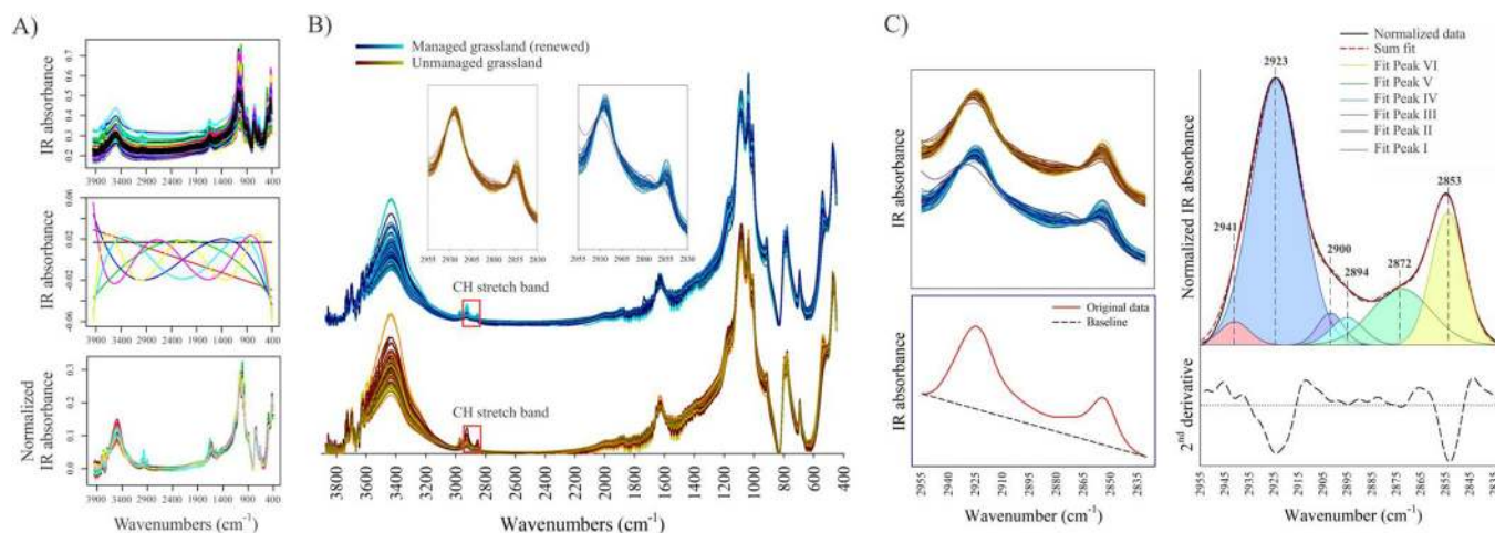
Fig. 3. FTIR spectral data processing of bulk soil samples from managed (renewed) and unmanaged grasslands. (A) Raw spectra; EMSC polynomials from 1 to 6 th and; normalized spectra. (B) Normalized spectra separated by soil management system – in evidence the CH stretch band. (C) Baseline corrections of the C–H vibrational region; spectral deconvolution guided by the position of the peaks obtained in the second derivative and; Gaussian curve fitting to semi-quantitative estimate of the peaks obtained by integrating the AUC.
