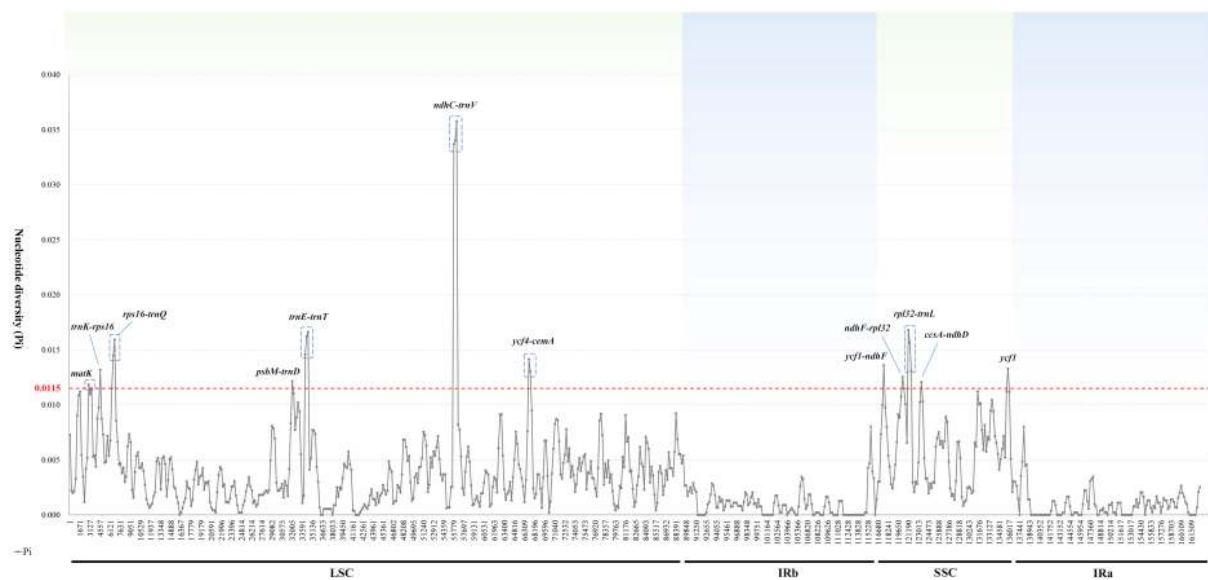
FIGURE 6 Sliding window analysis of the 16 Trollius plastomes. X-axis: position of the midpoint of a window; Y-axis: nucleotide diversity of each window.
