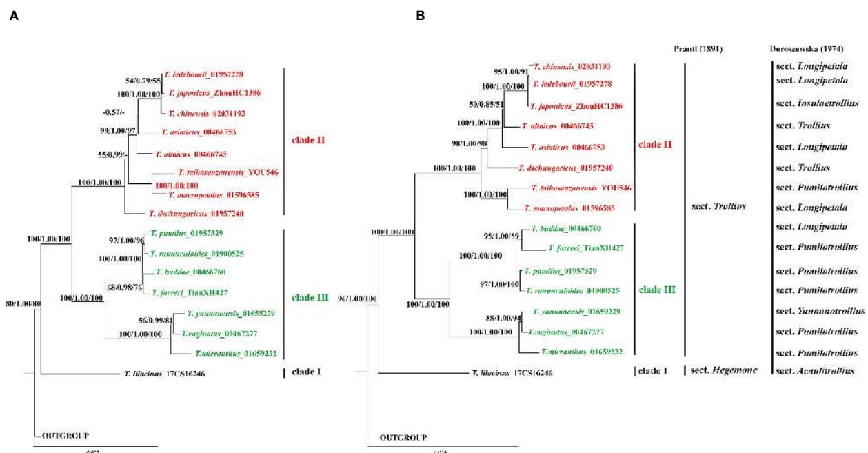
FIGURE 7 The phylogenetic tree of Trollius was reconstructed using maximum likelihood (ML), Bayesian inference (BI) and maximum parsimony (MP) methods. Each branch was annotated with three values: the ML bootstrap values, the Bayesian posterior probability, and the MP bootstrap values. (A) Phylogenetic tree constructed using the protein-coding sequences (CDS). (B) Phylogenetic tree constructed using the whole plastomes. Traditional classification systems of Prantl (1891) and Doroszewska (1974) were showed on the right vertical lines.
