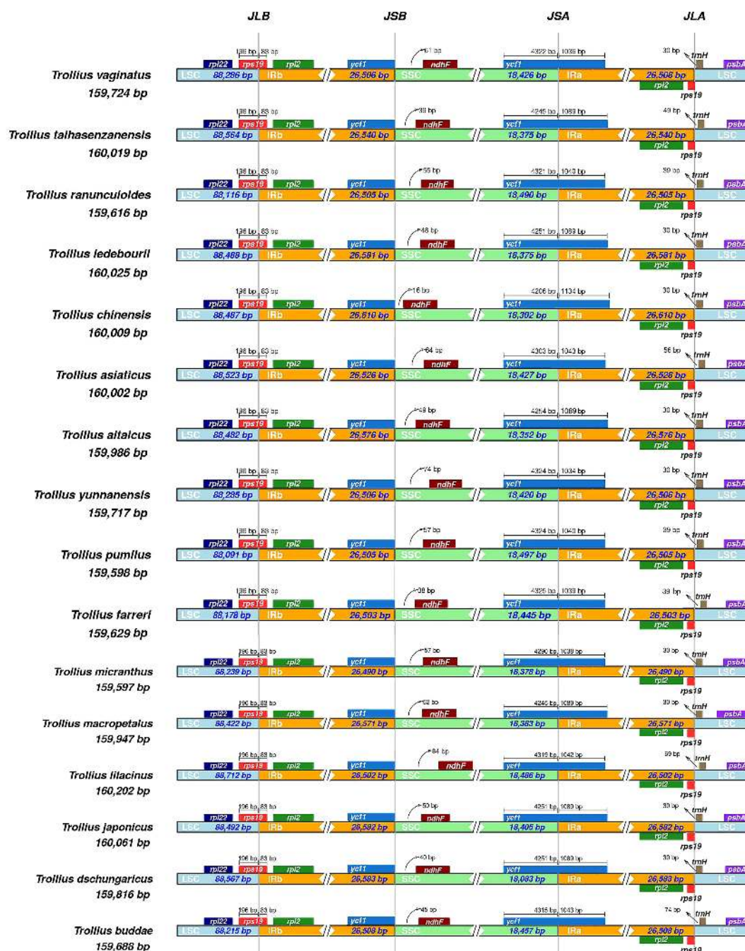
FIGURE 2 Comparison of the borders of LSC, SSC, and IR regions of plastomes in 16 Trollius species.
