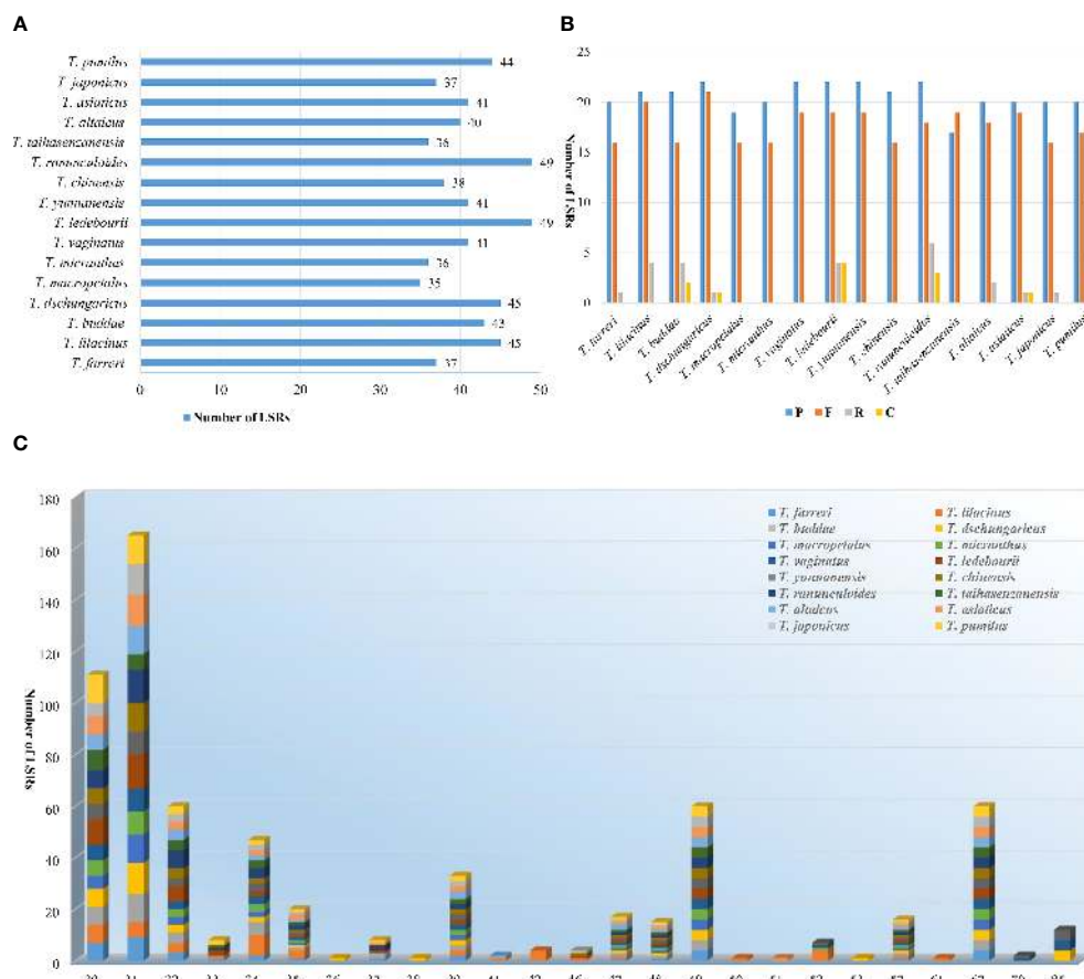
FIGURE 4 LSRs in the plastomes of 16 Trollius . (A) Number of LSRs. (B) Number of different LSRs types. (C) Number of LSRs of different lengths.
