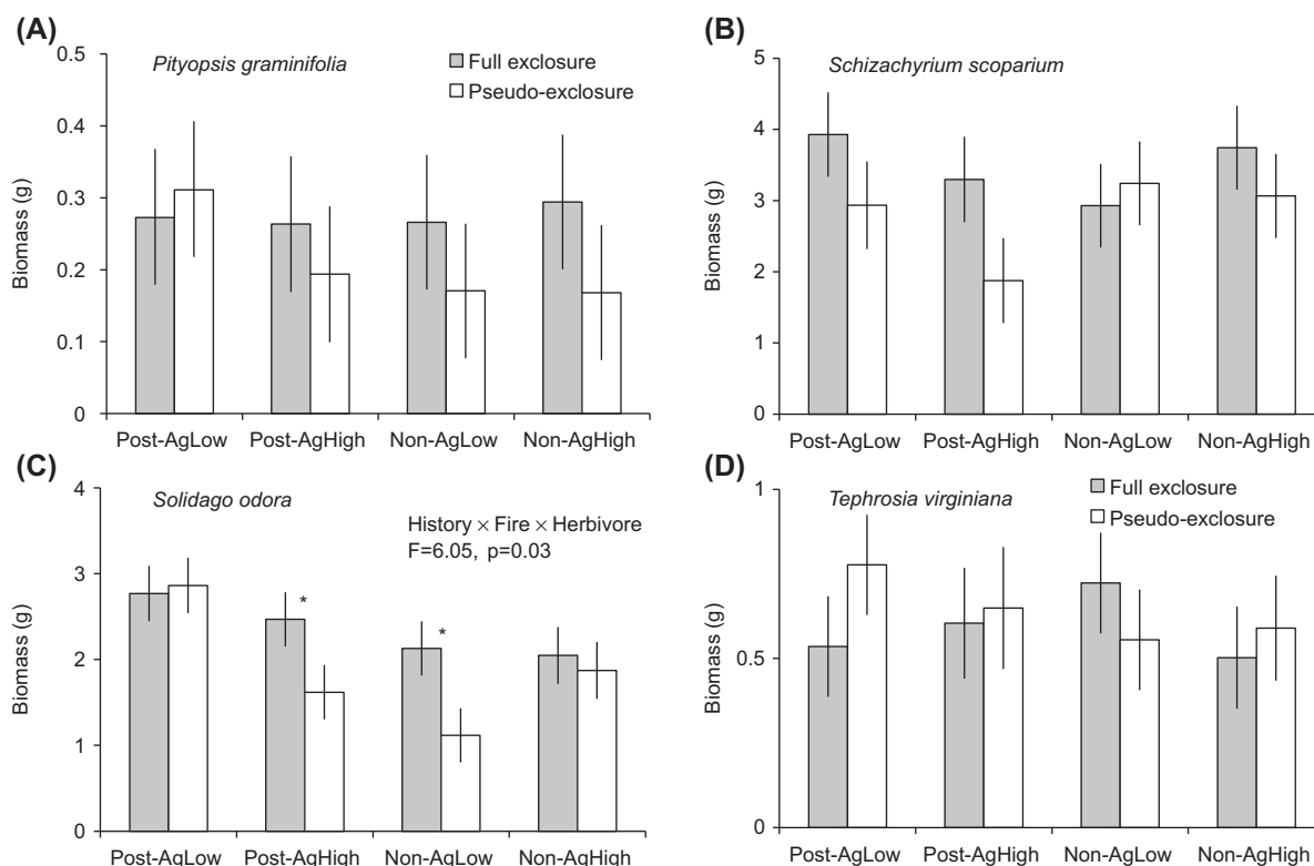
Figure 2. Biomass (g) at the end of the five week field experiment, after adjusting for initial plant height. Plants were protected from herbivores with mesh screen (Exclosure) or mesh screen with holes to allow invertebrate herbivores to enter (Pseudo-exclosure). Post-Ag = post-agricultural sites, Non-Ag = sites with no history of agriculture, Low = low fire frequency ( < 5 burns since 1991), High = high fire frequency ( \geq 5 burns since 1991). Significant ( p < 0.05 ) herbivore effects (i.e. factor × exclosure interactions) are listed on each panel. Asterisks (*) indicate significant ( p < 0.05 ) difference between exclosure and pseudo-exclosure treatments. Bars are \pm 1 SE. Note the value changes on the y-axis among the different species.
