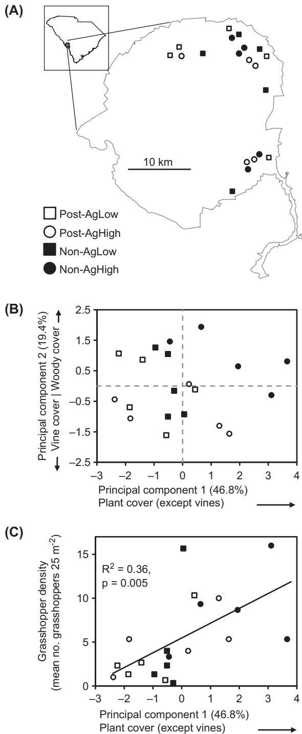
Figure 1. (A) Map of the study sites within the Savannah River Site, SC. (B) Principal component ordination of sites based on plant functional groups. Axis 1 explained 46.8% of the variability in the cover of six plant functional groups and represents an index of plant cover, particularly forb, grass, and legume cover. Axis 1 differed between land use histories ( p = 0.04 ) and fire frequency ( p = 0.02 ), but the interaction was not significant ( p = 0.30 ). (C) Grasshopper density response to herbaceous cover. The trend line and R^2 are for all treatments pooled. Post-Ag = post-agricultural sites, Non-Ag = sites with no history of agriculture, Low = low fire frequency ( < 5 burns since 1991), High = high fire frequency ( \geq 5 burns since 1991).
