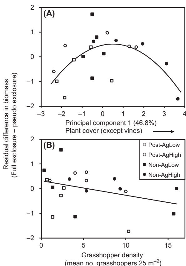
Figure 3. Effect of (A) the first principal component from the analysis of the plant community and its quadratic term and (B) grasshopper density on the (residual) difference in biomass between the full exclosure minus the pseudo-exclosure for Solidago odora . The full model included the principal component, the quadratic term of the principal component, and grasshopper density ( F = 4.90 , p = 0.01 , R^2 = 0.48 ). The graphs show each variable regressed against the residuals from a model containing the other term.
