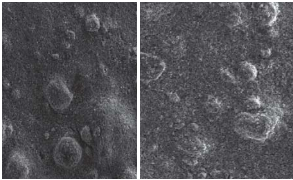
Fig. 4 SEM micrographs of fabricated \text{TiO}_2
