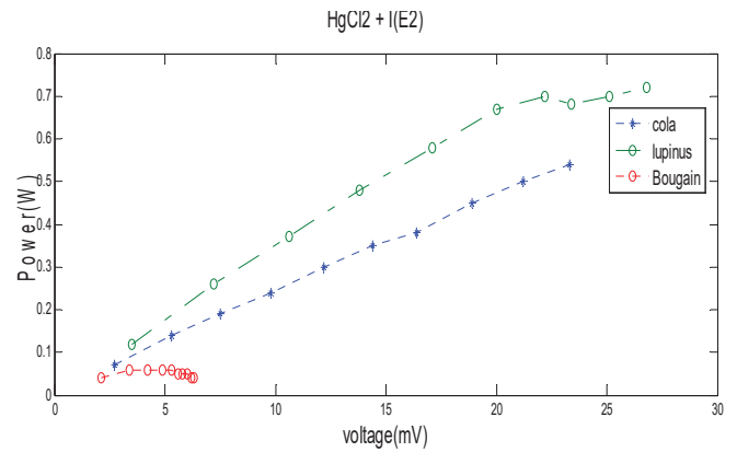
Fig. 6 I-V characteristics of DSSCs with C. acuminata , L. arboreus and B. spectabilis with electrolyte \text{HgCl}_2 + \text{I}
