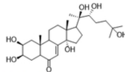
20-Hydroxyecdysone (3)
