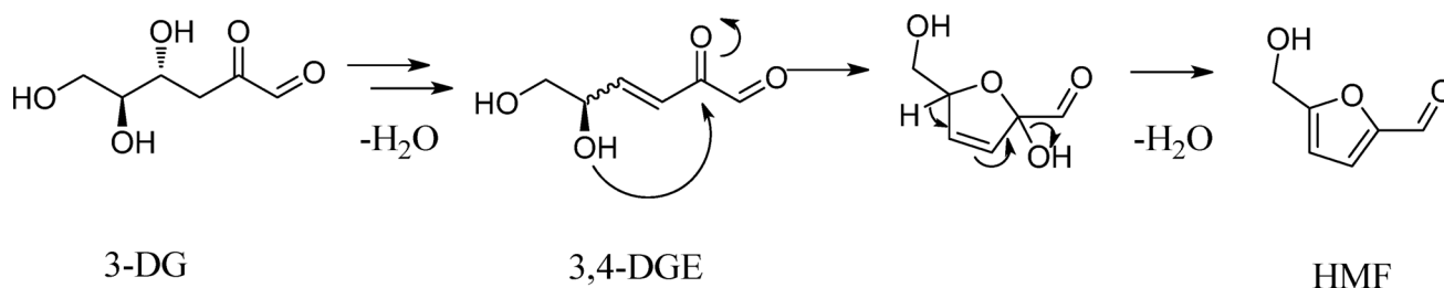
Fig. 1 Pathway of the formation mechanism of HMF
