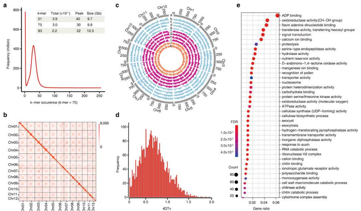
Extended Data Fig. 1 | The Taxus genomic features to complement Fig. 1. a, Genome size estimation of T. chinensis var. mairei based on k -mer distribution. The X-axis represents the occurrence of k -mers, and the Y-axis represents the frequency. The k -mer values for different genome sizes are shown in the inner table. b, Genome-wide all-by-all Hi-C interaction. The heat map shows Hi-C interactions under a resolution of 2 Mb. Darker red pixels indicate higher contact probabilities. The number on the scale bar indicates the number of links after logarithmic analysis. c, Genomic landscape of the twelve pseudochromosomes. Track a represents the length of the pseudochromosomes (Mb); b, c, d, and e show the expression of tissue-specific genes in the bark of stem, root, strobili and leaf from the male Taxus plant, respectively; f, g, h, and i show the expression of tissue-specific genes in the bark of stem, root, strobilus and leaf from the female Taxus plant, respectively; j and k display high- and low-producing paclitaxel cell lines, respectively. d, Whole genome duplication (WGD) analysis based on the substitution rate distribution of paralogs. The 4DTV values of paralogs were calculated using KaKs _calculator with the YN model. The X-axis is the value of fourfold synonymous third-codon transversions (4DTV) for paralogous pairs in the Taxus genome, and the Y-axis represents the frequency. e, Gene Ontology (GO) enrichment for gene families with significant expansion. GO enrichment analysis of a subset of 142 gene families with significant expansion ( p < 0.05 ); FDRs were adjusted for multiple testing. The size and color of dots indicate the number of genes and false discovery rate (FDR), respectively. The X-axis represents the gene ratio, and the GO terms are listed on the Y axis.
