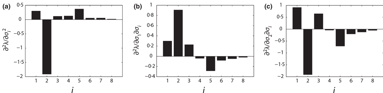
Fig. 3. Three sets of second derivatives from H[\lambda; \sigma] (Figure 2). (a) The pure second derivatives \partial^2 \lambda / \partial \sigma_i^2 . (b) The mixed second derivatives \partial^2 \lambda / \partial \sigma_i \partial \sigma_j . (c) The mixed second derivatives \partial^2 \lambda / \partial \sigma_i \partial \sigma_j .
