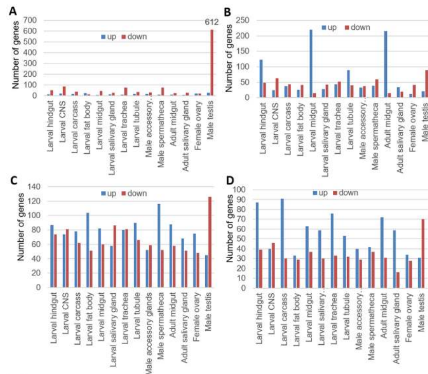
Fig 9. Tissue-specificity of genes that were differentially expressed in juvenile hormone analog (JHA)- and disruptor (JHD)-fed D. melanogaster larvae. The genes significantly activated by JHA and significantly repressed by JHD (S2 Table) were applied to gene expression database constructed using Affymetrix microarray results to characterize tissue-specific expression. (A) Tissue-specificity of JHA \uparrow JHD \downarrow genes which were significantly activated by JHA and significantly repressed by JHD; (B) Tissue-specificity of JHA \downarrow JHD \uparrow genes which were significantly repressed by JHA and significantly activated by JHD; (C) Tissue-specificity of JHA \uparrow JHD \uparrow genes which were significantly activated by both JHA and JHD; and (D) Tissue-specificity of JHA \downarrow JHD \downarrow genes which were significantly repressed by both JHA and JHD.
