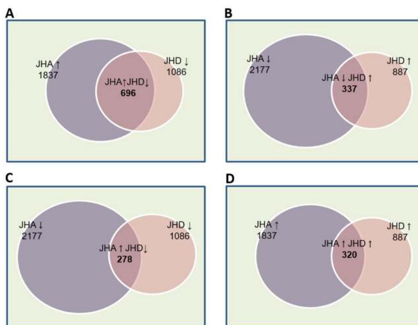
Fig 7. Transcriptome analysis of genes that were differentially expressed in juvenile hormone analog (JHA, methoprene)- and disruptor (JHD, methyl lucidone)-treated Drosophila melanogaster larvae. JHA \uparrow , genes significantly activated by JHA treatment; JHA \downarrow , genes significantly repressed by JHA treatment; JHD \uparrow , genes significantly activated by JHD treatment; JHD \downarrow , genes significantly repressed by JHD treatment. (A) JHA \uparrow JHD \downarrow , genes significantly activated by JHA and significantly repressed by JHD; (B) JHA \downarrow JHD \uparrow , genes significantly repressed by JHA and significantly activated by JHD; (C) JHA \downarrow JHD \downarrow , genes significantly repressed by both JHA and JHD; and (D) JHA \uparrow JHD \uparrow , genes significantly activated by both JHA and JHD.
