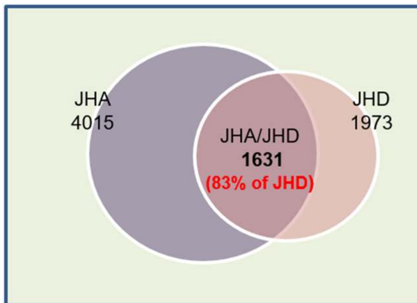
Fig 6. Illumina RNA-seq transcriptome analysis of juvenile hormone analog (JHA, methoprene)- and disruptor (JHD, methyl lucidone)-treated Drosophila melanogaster larvae. JHA, genes significantly affected by JHA; JHD, genes significantly affected by JHD; JHA/JHD, genes significantly affected by both JHA and JHD; JHA \uparrow , genes significantly activated by JHA; JHD \downarrow , genes significantly repressed by JHD; JHA \uparrow JHD \downarrow , genes significantly activated by JHA and significantly repressed by JHD.
