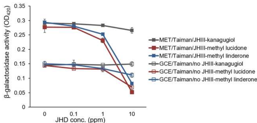
Fig 4. Juvenile hormone disruptor (JHD) activities of three Lindera erythrocarpa diterpenes against Met-Taiman and GCE-Taiman binding. Dose-dependent inhibition of pyriproxyfen-mediated Met-Taiman binding or constitutive GCE-Taiman binding was observed for two L. erythrocarpa JHD diterpenes, i.e., methyl lucidone and methyl linderone. Kanagugiol did not significantly disrupt either Met-Taiman or GCE-Taiman binding. Values and error bars indicate means \pm SD ( n = 4 ).
