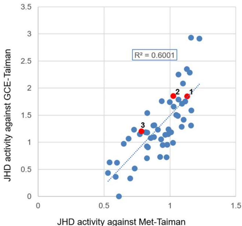
Fig 2. Juvenile hormone disruptor (JHD) activity of 53 plant species against Met-Taiman and GCE-Taiman binding. The JHD activities of 53 high-JHD plant species against Met-Taiman and GCE-Taiman binding were calculated as the average JHD activity of four independent experiments. Values in the rectangular box indicate the coefficients of determination ( R^2 ) for JHD activity of Met-Taiman and GCE-Taiman binding. 1, Lindera erythrocarpa ; 2, Pinus densiflora ; 3, Solidago serotina .
