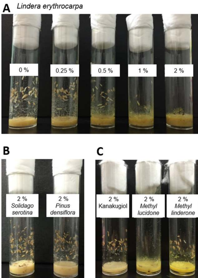
Fig 3. Effect of Lindera erythrocarpa , Solidago serotina , and Pinus densiflora extracts and three juvenile hormone disruptor (JHD) diterpenes from L. erythrocarpa on the larval development of Drosophila melanogaster . (A) Effect of L. erythrocarpa on the development of D. melanogaster larvae at a concentration-dependent manner. (B) Effect of 2% (w/v) S. serotina and P. densiflora extracts on the development of D. melanogaster larvae. (C) Effect of 2% (w/v) methyl lucidone, a JHD diterpene from L. erythrocarpa , on the development of D. melanogaster larvae.
