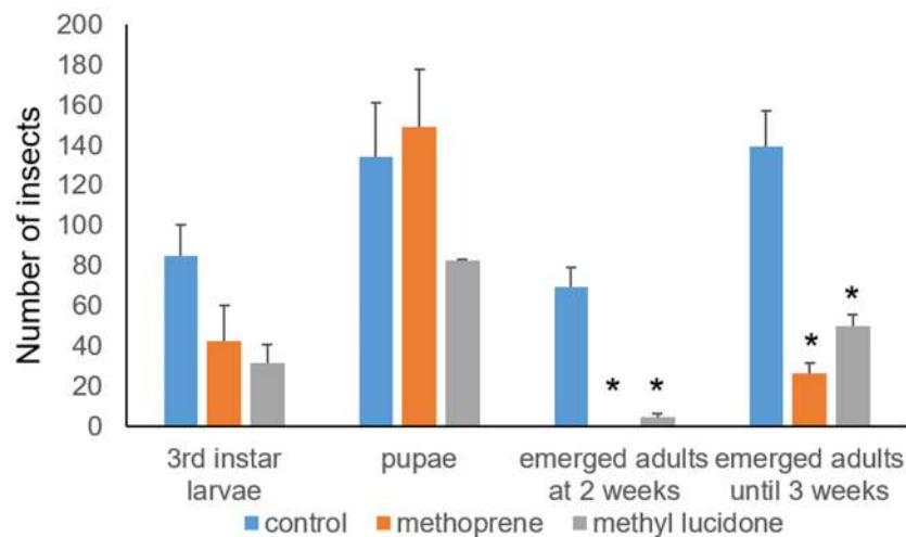
Fig 5. Larval and pupal development of Drosophila melanogaster fed sublethal doses of juvenile hormone analog (JHA) or disruptor (JHD). Values and error bars indicate means \pm SD ( n = 3 ). *, p < 0.05 ( t -test).
