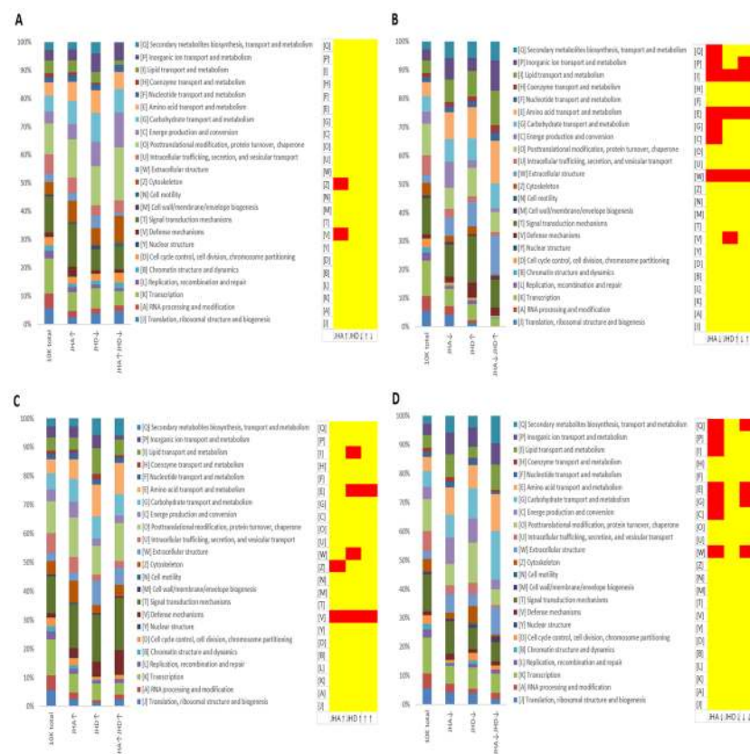
Fig 8. Gene ontology analysis of gene cohorts that were differentially expressed in juvenile hormone analog (JHA)- and disruptor (JHD)-fed D. melanogaster larvae. Red indicates ontology groups with significant overrepresentation ( P < 0.01 in a hypergeometric distribution). The functional groups with corresponding abbreviations and colors are indicated. (A) JHA \uparrow JHD \downarrow , genes significantly activated by JHA and significantly repressed by JHD; (B) JHA \downarrow JHD \uparrow , genes significantly repressed by JHA and significantly activated by JHD; (C) JHA \uparrow JHD \uparrow , genes significantly activated by both JHA and JHD; and (D) JHA \downarrow JHD \downarrow , genes significantly repressed by both JHA and JHD.
