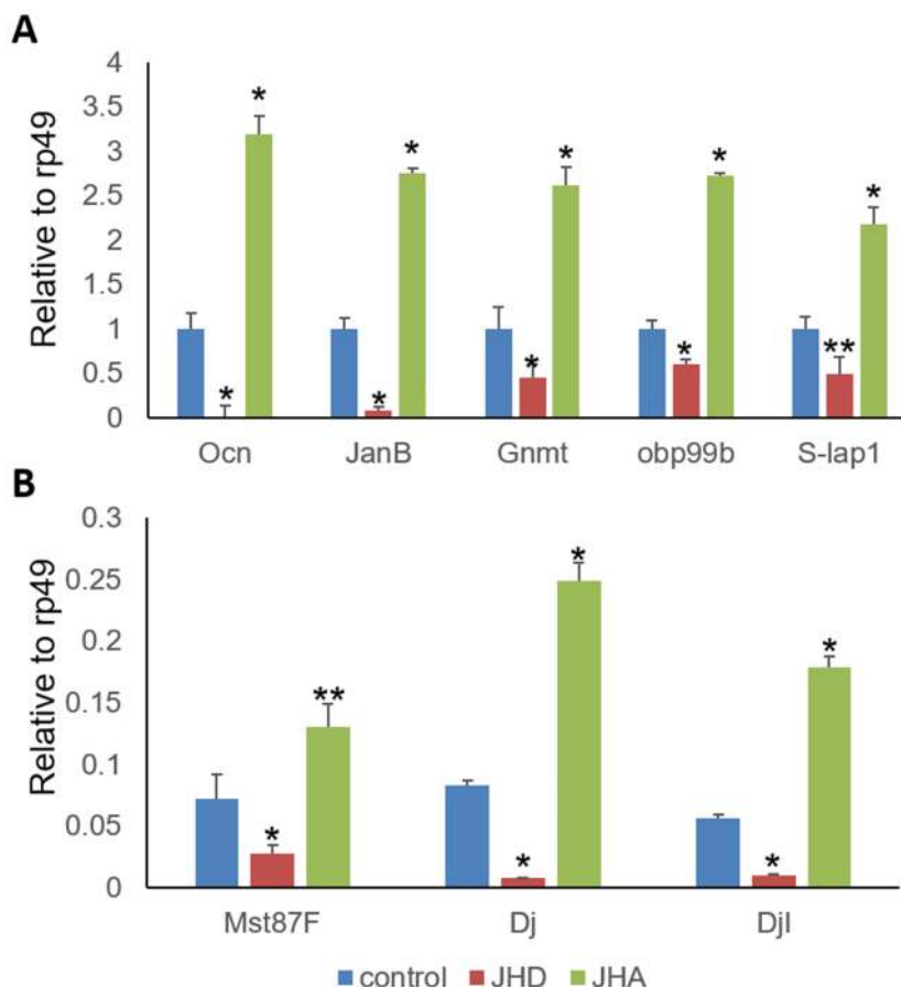
Fig 10. Validation of genes significantly activated by juvenile hormone analog (JHA) and significantly repressed by juvenile hormone disruptor (JHD). (A) JHD- or JHA-dependent regulation of five randomly selected JHA \uparrow JHD \downarrow genes: ocnus ( ocn ), janus B ( janB ), Glycine N-methyltransferase ( Gnmt ), Odorant-binding protein 99b ( Obp99b ), and Sperm-Leucylaminopeptidase 1 ( S-Lap1 ). (B) JHD- or JHA-dependent regulation of three tTAF-dependent JHA \uparrow JHD \downarrow genes: Male-specific RNA 87F ( Mst87F ), don juan ( dj ), and don juan-like ( djl ). Total RNA was extracted from the wandering third-instar larvae that were fed ethanol (control)-, methoprene (JHA)-, or methyl lucidone (JHD)-supplemented diet and analyzed using qPCR. Values and error bars indicate means \pm SD ( n = 3 ). *, p < 0.01 and **, p < 0.05 ( t -test).
