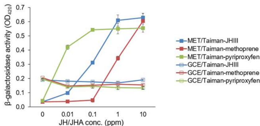
Fig 1. Microplate simulation of juvenile hormone III (JH III)- or juvenile hormone analog (JHA)-dependent Met-Taiman or GCE-Taiman binding. Yeast Y197 cells were transformed using yeast two-hybrid (Y2H) plasmids that contained Met-Taiman or GCE-Taiman and were incubated with different concentrations of JH III or JHAs. The JH III/JHA-mediated binding of Met-Taiman and GCE-Taiman was measured by absorbance values at 420 nm ( OD_{420} ) after assaying \beta -galactosidase activity. Values and error bars indicate means \pm SD ( n = 3 ).
