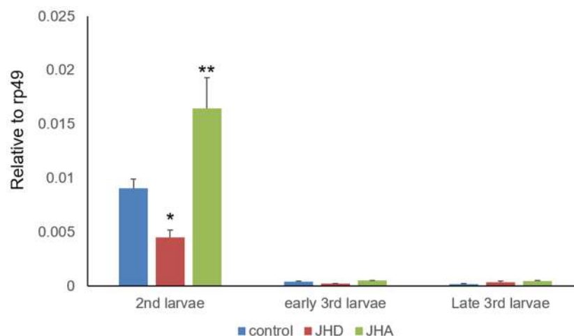
Fig 11. Stage-specific regulation of Krüppel homolog 1 ( Kr-h1 ) by juvenile hormone analog (JHA) and disruptor (JHD). Total RNA samples were prepared from second-, early third-, and wandering third-instar larvae fed ethanol (control)-, methoprene (JHA)-, or methyl lucidone (JHD)-supplemented diets and analyzed using qPCR. Values and error bars indicate means \pm SD ( n = 3 ). *, p < 0.01 and **, p < 0.05 ( t -test).
