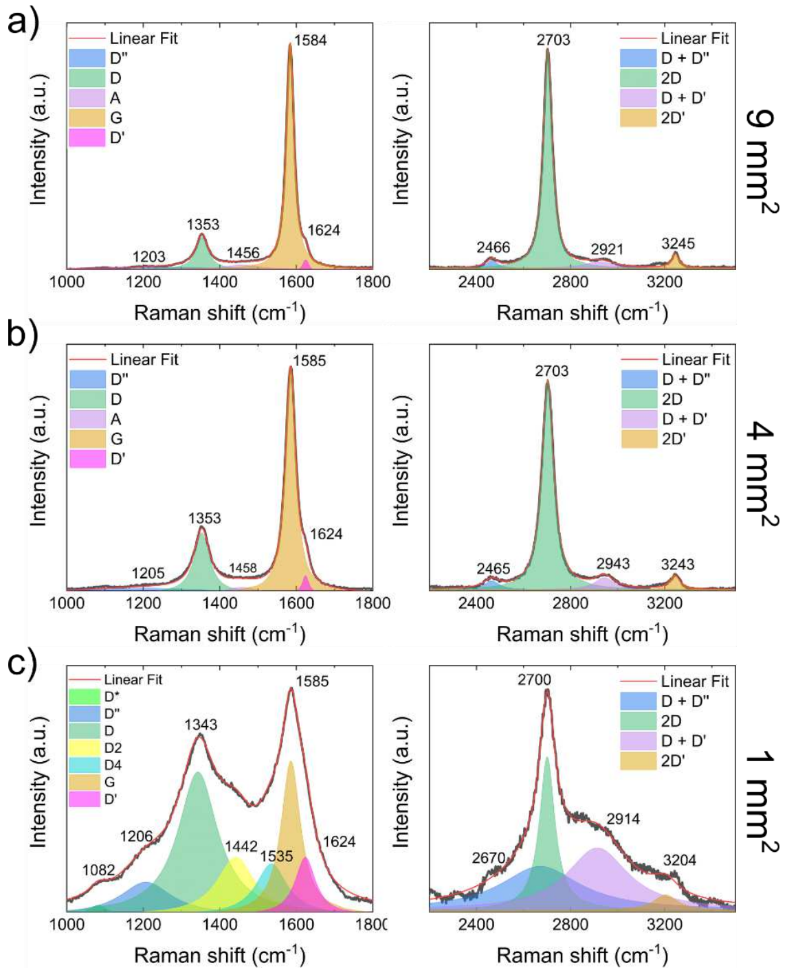
Figure 6. Fitting the Raman spectrum corresponding to samples with an irradiation area of 9 mm 2 , 4 mm 2 , and 1 mm 2 .
