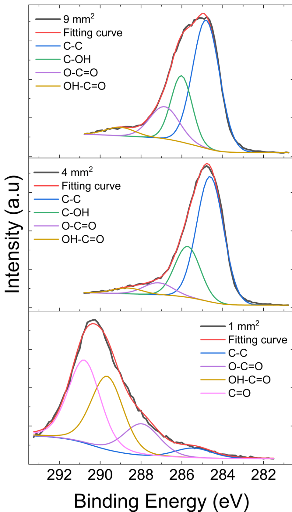
Figure 8. High-resolution C 1s XPS spectra of T-80 samples synthesized at irradiation areas of (a) 9 mm 2 , (b) 4 mm 2 , and (c) 1 mm 2 , illustrating the evolution from dominant sp 2 carbon to increased sp 3 and oxygenated species at smaller irradiation areas.
