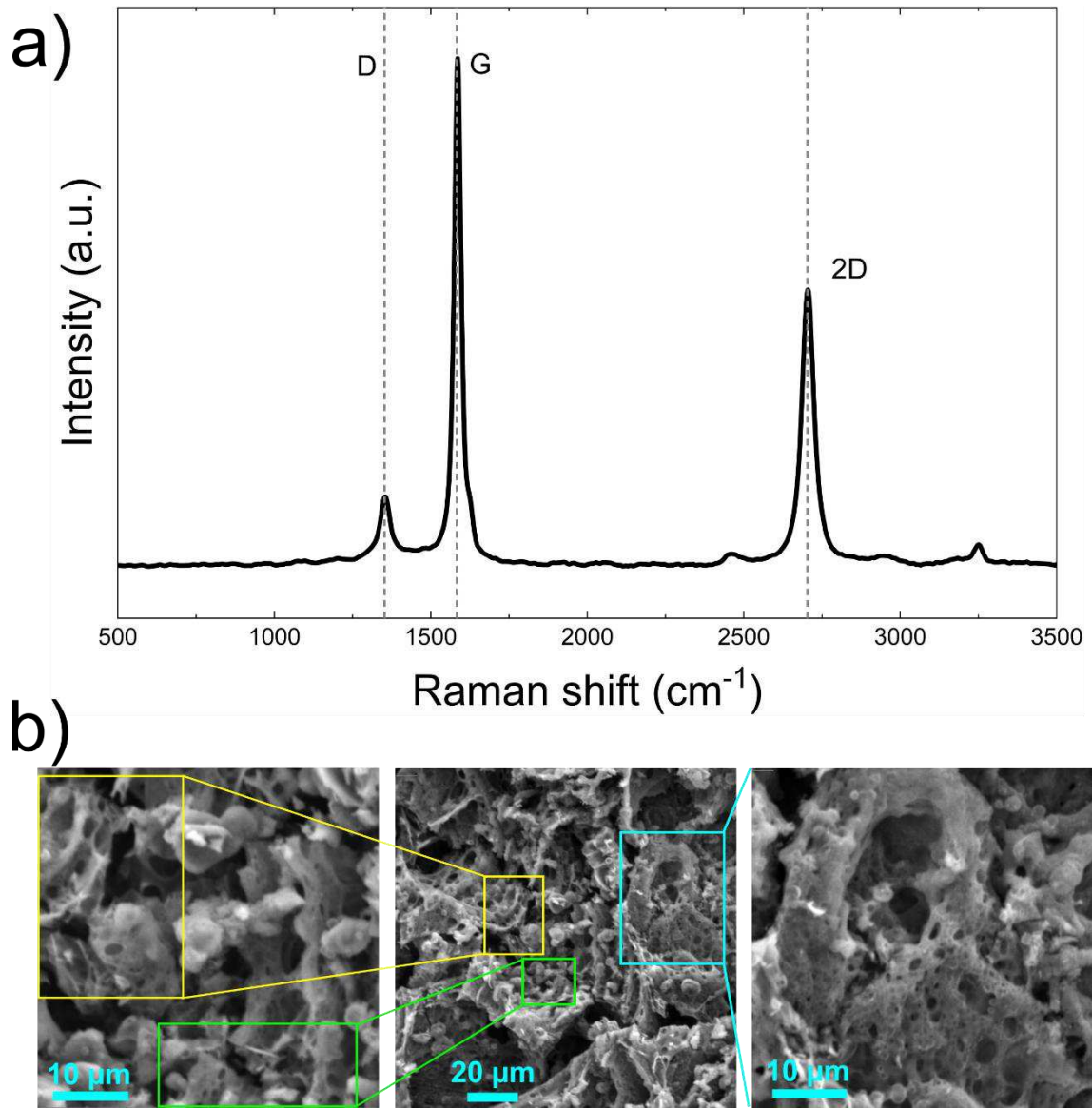
Figure 9. LIG was synthesized with a laser power of 11%, at 50 mm s -1 with a defocus distance of 9 mm. (a) Ramana spectrum of a representative sample of the LIG synthesis. (b) SEM images (1000×) of the irradiated regions showing surface morphology.
