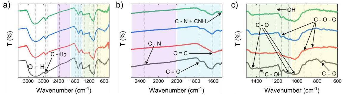
Figure 7. FTIR spectra of untreated avocado seed powder and LIG samples synthesized from T-80 powder with irradiation areas of 9, 4, and 1 mm 2 , showing the evolution of oxygen-containing functional groups after laser processing.
