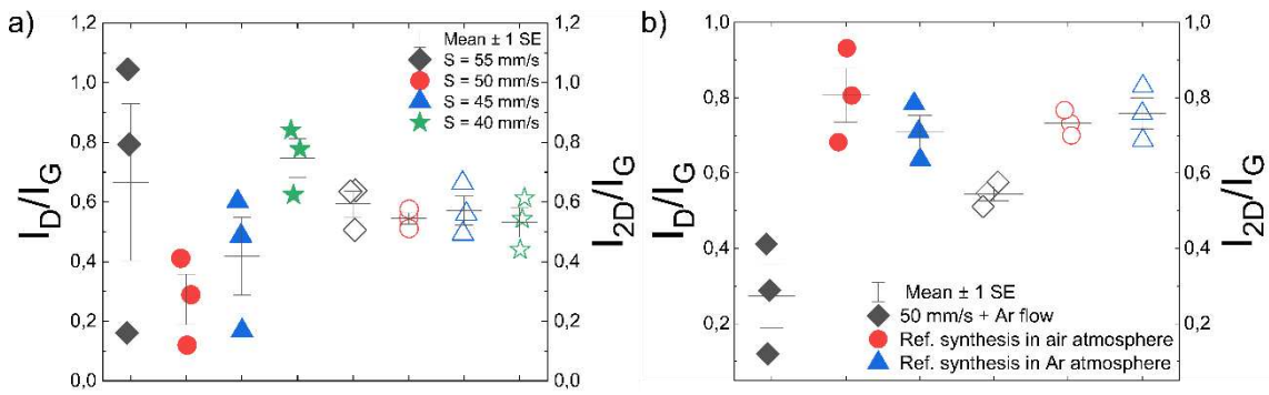
Figure 3. Effect of scan speed and processing atmosphere on the structural quality of LIG. (a) I_D/I_G and I_{2D}/I_G ratios for samples synthesized at different scan speeds (10% laser power, 4\text{ mm}^2 area). (b) Comparison of Raman intensity ratios for samples synthesized in ambient air and under argon flow at Reference [32].
