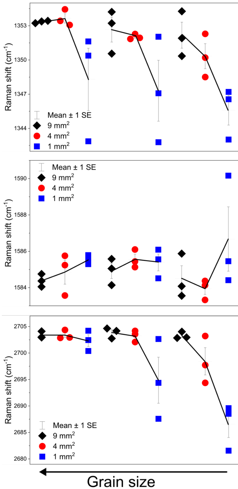
Figure 5. Variation in Raman band positions (D, G, and 2D) as a function of irradiation area and particle size, illustrating structural evolution and changes in graphene layer stacking.
