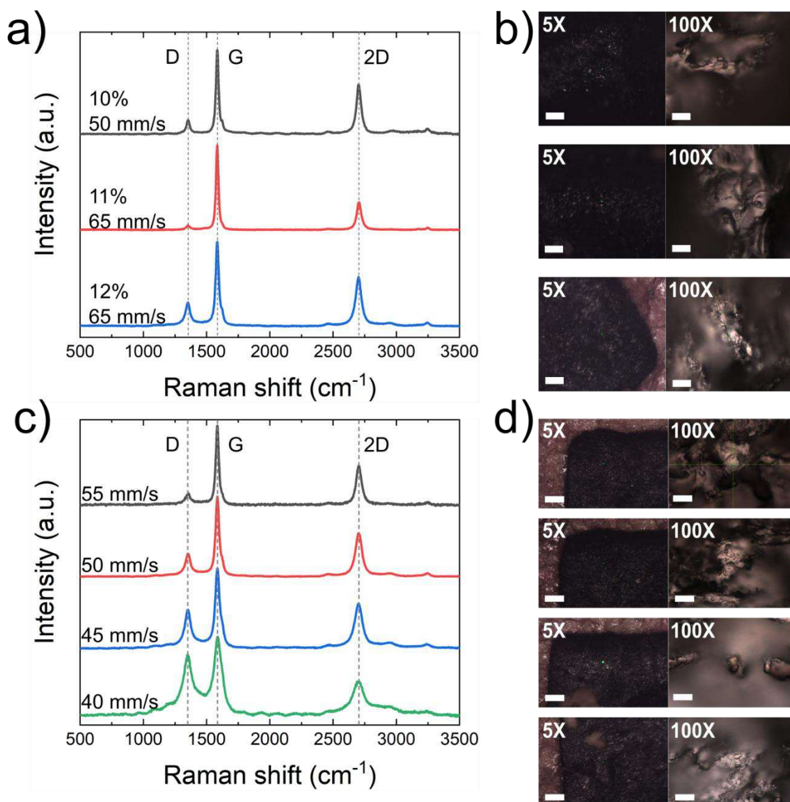
Figure 2. Influence of laser power and scan speed on LIG formation from T-80 avocado seed pellets. (a) Raman spectra of samples processed at different laser powers and scan speeds. (b) Optical micrographs showing morphological degradation at higher laser
