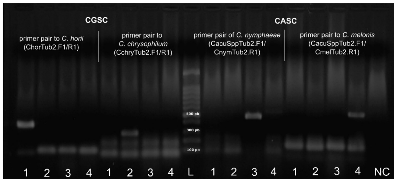
Fig. 3 Agarose gel electrophoresis of PCR products from isolates of Colletotrichum spp., causal agents of persimmon anthracnose, using specific primers. Samples 1 to 4 represent isolates DkCPR18-03 ( C.
