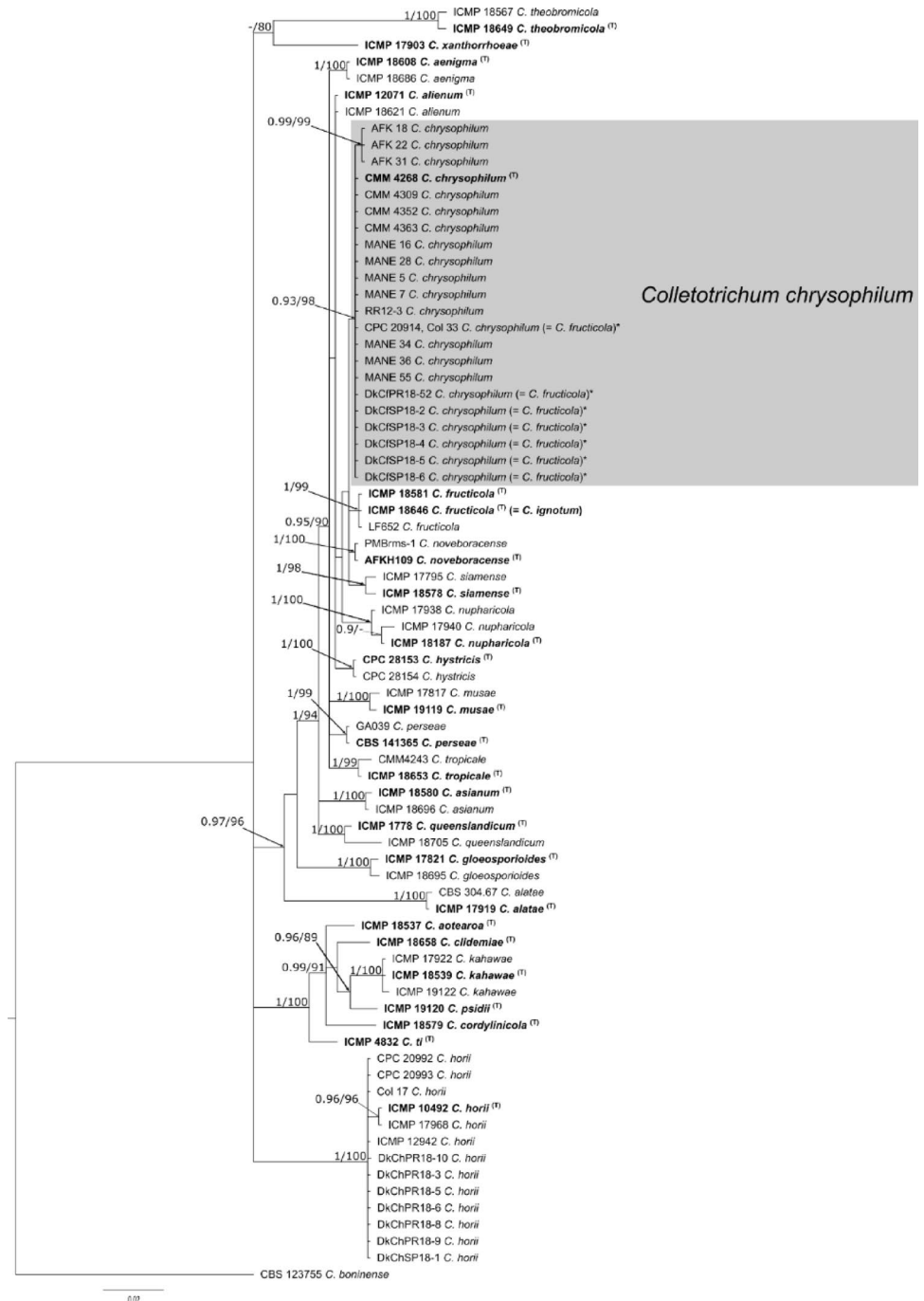
Fig. 1 Bayesian Inference phylogenetic tree of the Colletotrichum gloeosporioides species complex (CGSC) based on concatenated sequences of the ITS-rDNA region and the partial genes GAPDH and TUB2 . Colletotrichum isolates re-evaluated in this study are marked with (*) and identified as C. chrysophilum (previous identification in parentheses – C. fructicola ). Other sequences were obtained from the NCBI database, with type strains highlighted in bold and indicated with superscript (T). Posterior probability (PP) values greater than 0.9 and ultrafast bootstrap support (UFBoot) values greater than 80 are shown at branch nodes (PP/UFBoot). A hyphen (-) indicates support values below the predefined thresholds for the analyses. The scale bar represents the estimated number of substitutions per nucleotide. The phylogenetic tree is rooted with C. boninense CBS 123,755, which was used as the outgroup for the CGSC
