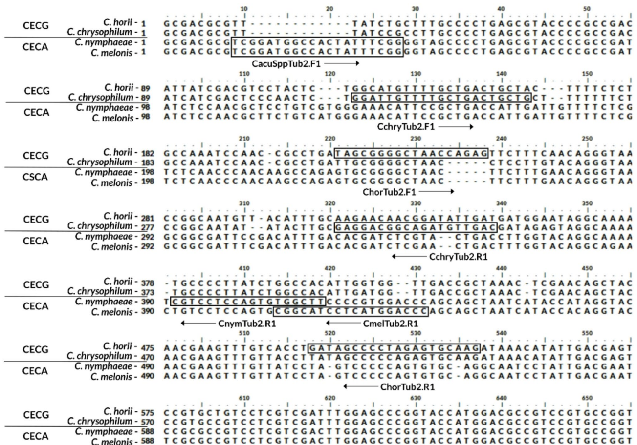
Fig. 2 Comparison of genomic DNA sequences of the partial TUB2 gene from isolates belonging to the Colletotrichum gloeosporioides species complex (CGSC): C. horii (DkCPR18-03, MN982451) and C. chrysophilum (DkCSP18-06, MK209630); and to the Colletotri-
