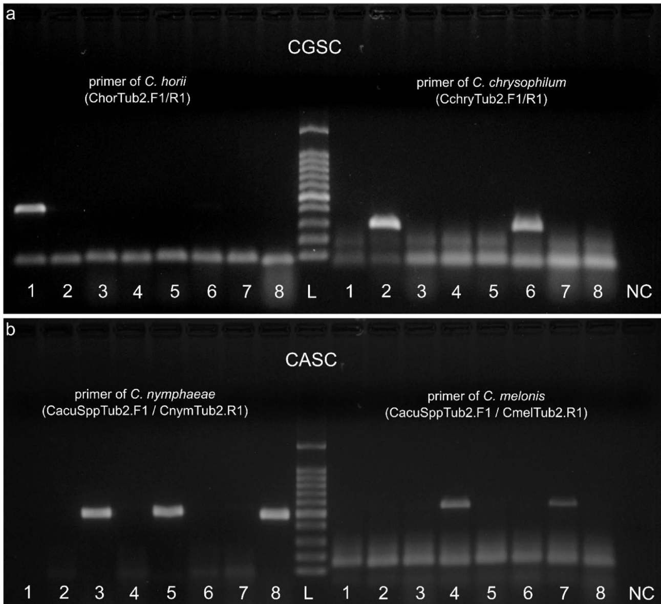
Fig. 5 Agarose gel electrophoresis of PCR products from Colletotrichum spp. isolates. of persimmon, apple and pear trees. Samples 1 to 8 represent isolates DkCPR18-03 ( C. horii from persimmon tree), DkCSP18-06 ( C. chrysophilum from persimmon tree), DkCPR18-01 ( C. nymphaeae from persimmon tree), DkCPR18-11 ( C. melonis from persimmon tree), Col 15 ( C. nymphaeae from apple tree), Col
