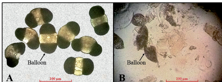
Figure 5. Pine pollen ( Pinus halepensis ) observed under optical light microscopy, (200x magnification) from Brazdova et al . [157]. A: Intact pollen grains. B: Grinded pollen using a multidirectional grinder (fast-prep 24-5G, cool prep, MPBiomedicals) in the presence of 1 mm silica beads. The disruption of pollen grains results in qualitative and quantitative enriched protein extraction.
