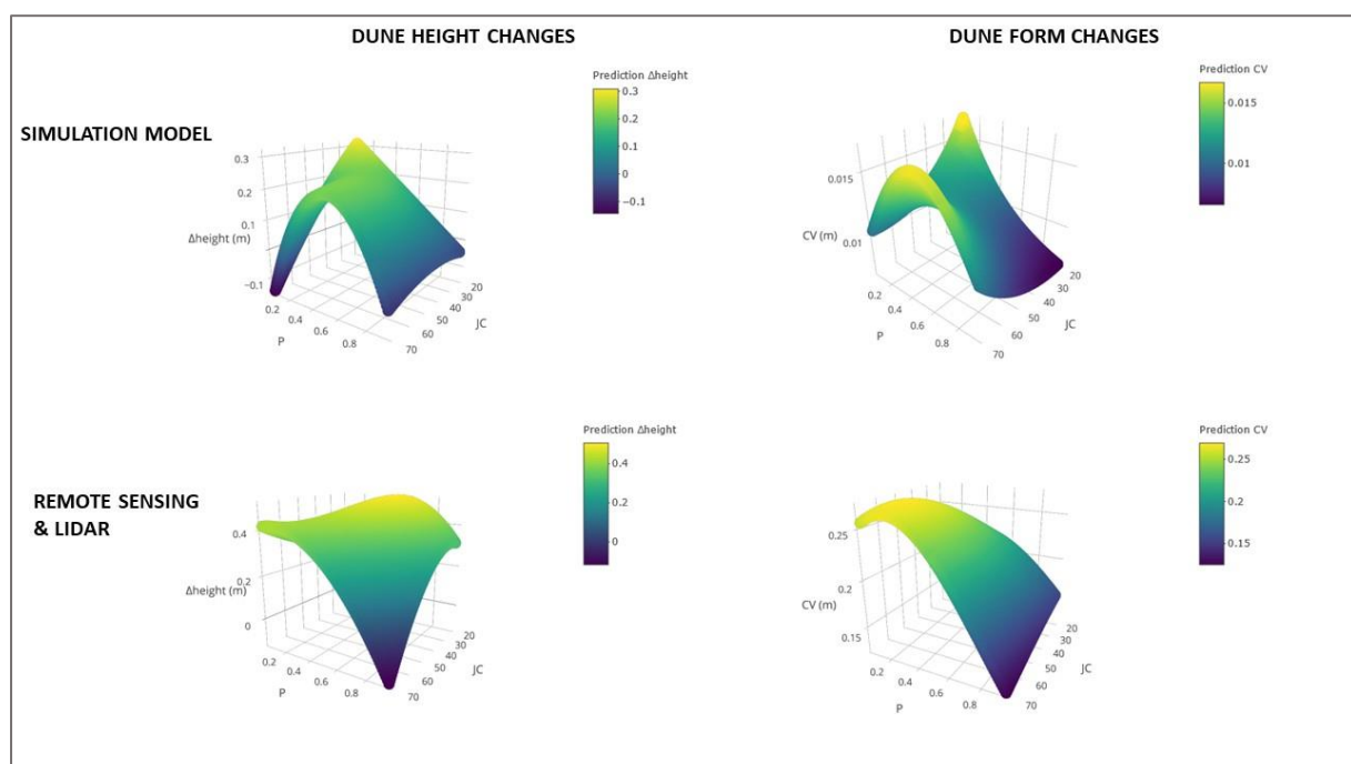
Figure 5. Output of the simulations computing changes in dune height and topography (CV of height changes over all grid cells) over a period of 5 years (upper panel), and similar metrics as observed from LiDAR data from coastal dunes along the Belgian west coast (lower panels).
