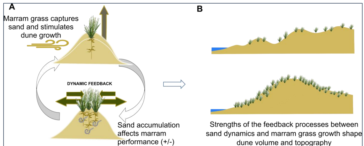
Figure 1. Conceptual figure on the role of marram grass as an engineer in foredune formation. A. Once established, the species' sand capture ability shapes local sand accumulation, leading to an increase in dune volume. This sand accumulation will promote the species' growth, unless burial is too severe. If sand accumulation ceases, either due to decreased input from the sea, or to sheltering effects from surrounding vegetation, the plant performance will decrease due to pathogen accumulation in the roots, after which marram grass will degenerate. B. These dynamic feedbacks depend on the species' spatial configuration and external environmental conditions and will eventually shape the development of its volume and form, and, hence, its stability and resilience against storm surges under climate change.
