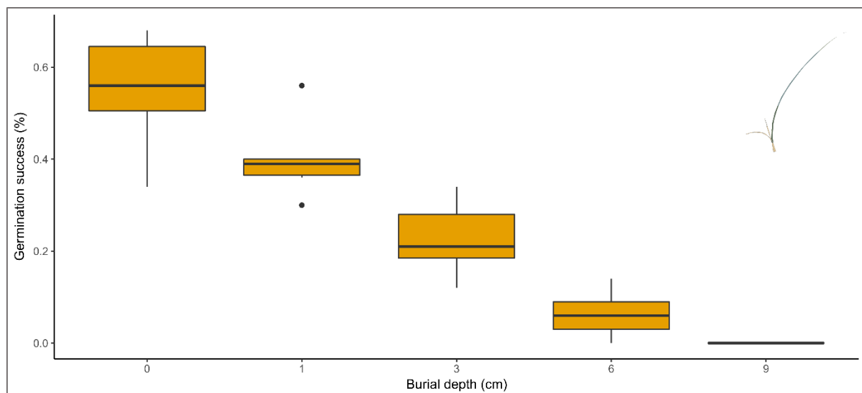
Figure 2. Seedling emergence in relation to sand burial (see supplement1)
