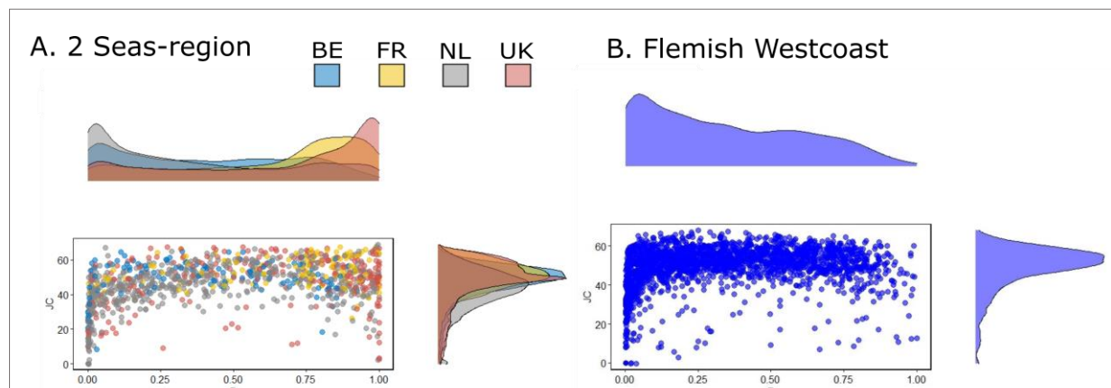
Figure 3. Density distribution plots of observed cover (P) and spatial correlation (JC) of marram grass in 20x20 m 2 grid cells in dunes from the Isles of Scilly to Norfolk in England (UK) and from Somme (Fr) to Texel (NL) on the continental side along the North Sea and the Flemish West coast (B) (right panel). Note that for visualisation, a subsampling of 1000 points (2%) was performed for (A).
