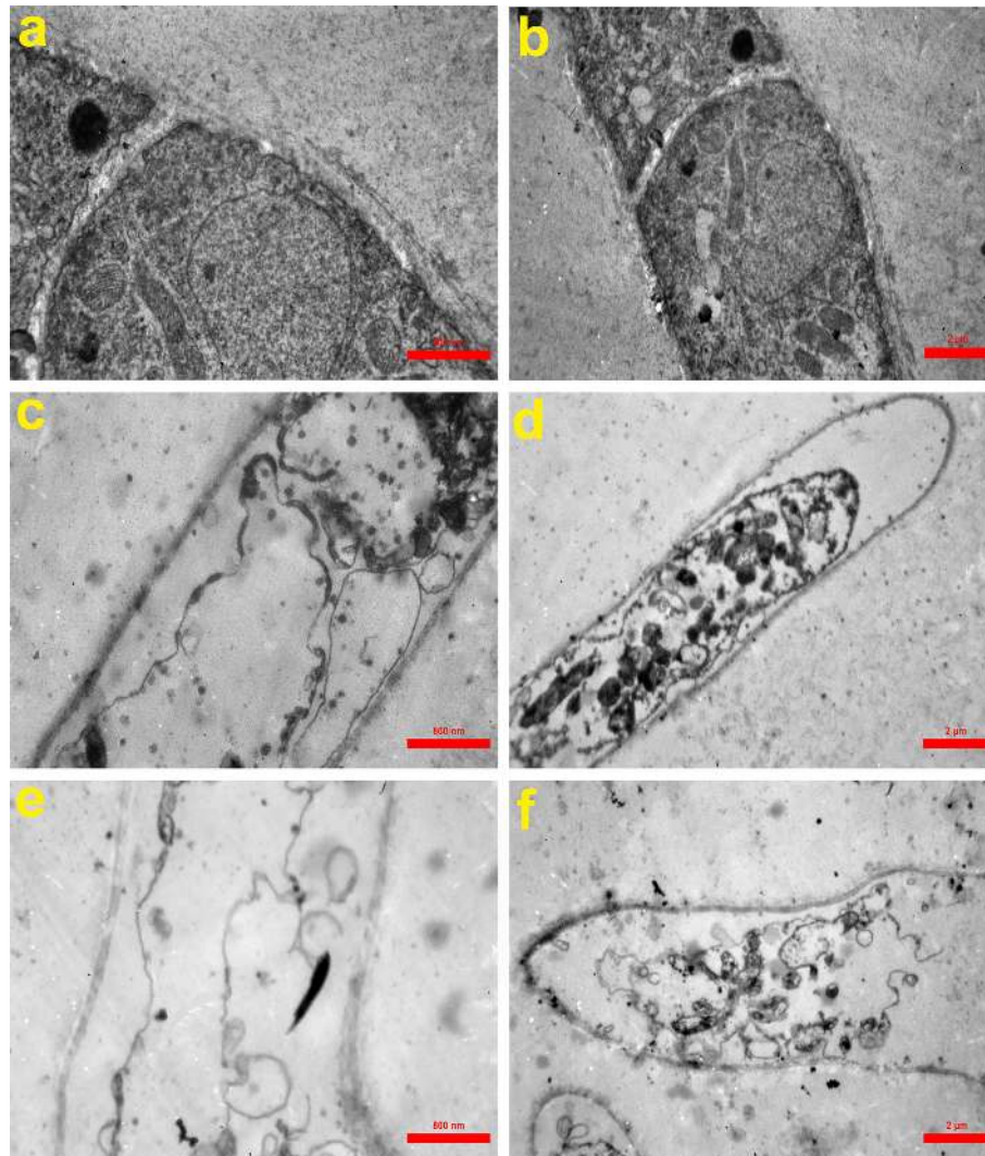
FIGURE 6 | Transmission electron microscopy of A. fumigatus -untreated hyphae (A, B) and hyphae exposed to Cc-AFP1 at the concentrations of 16 µg/ml (C, D) and 32 µg/ml (E, F). Untreated hyphae of A. fumigatus had intact cell walls, integrated cell membranes, and normal organelles (A, B). In contrast, in treated hyphae with Cc-AFP1, pathologic ultrastructure changes including attenuated irregular cell wall, loss of the structural integrity and shrinkage of the cell membrane, detachment of the cell membrane from the cell wall, cytoplasmic depletion, and membranous damage of cytoplasmic organelles especially mitochondria were evident (C–F).
