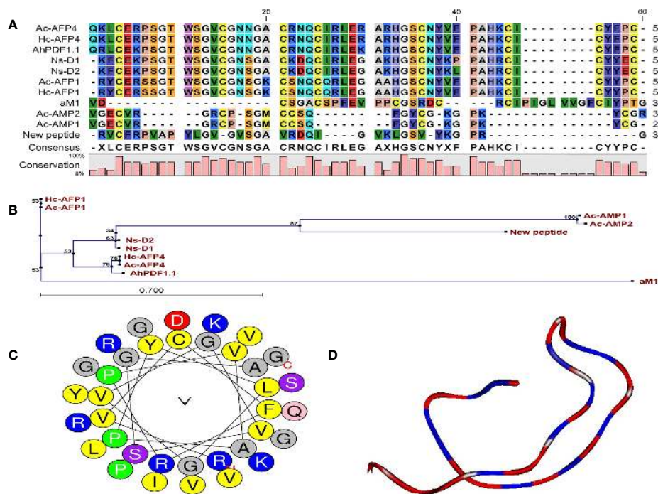
FIGURE 3 | Characteristic features and structural data of Cc-AFP1. (A) The alignment of Cc-AFP1 amino acid sequences as well as the sequences related to other antimicrobial peptides. (B) Phylogenetic tree of Cc-AFP1. Phylogenetic tree was acquired by CLC main workbench software. Each sequence name is written at the end of the relevant branch. The tree reliability was determined using bootstrap method with 100 replications. (C) Helical wheel diagram of Cc-AFP1 peptide and polar and non-polar amino acids, and their locations in peptide can be observed. (D) Three-dimensional structure model of The Cc-AFP1 with random coil.
