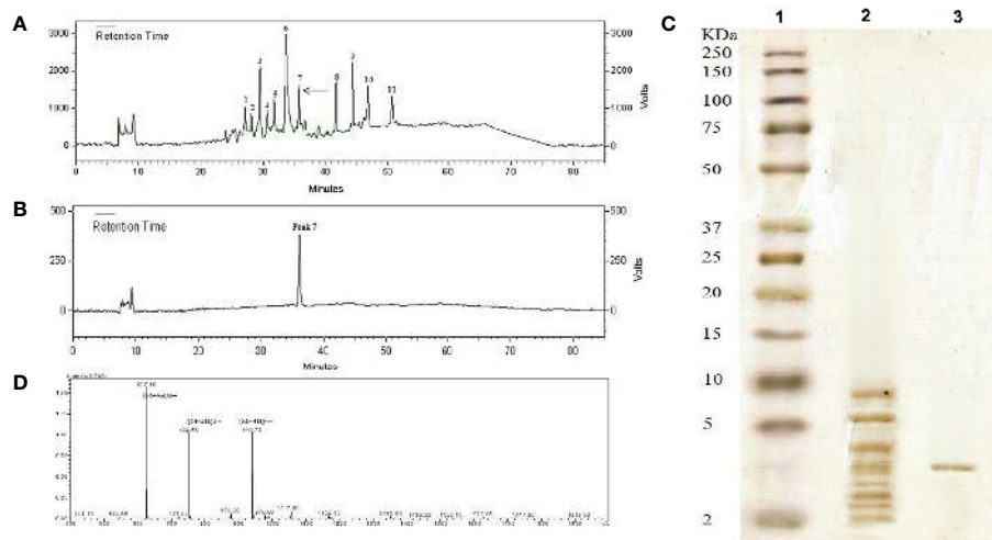
FIGURE 1 | (A) Peptide RP-HPLC purification from Carum carvi seeds. The arrow shows the active peak 7. (B) The chromatogram obtained after the re-chromatography process to purify the active peak 7. (C) Tricine-SDS-PAGE profile stained with silver (1) molecular weight markers (2–250 kDa), (2) the extracted peptide passing through an ultra-membrane with the cutoff of 10 kDa, and (3) the RP-HPLC column purified peak 7. (D) ESI- mass spectrum of purified antifungal peptide. Multiple charged molecular ions are indicated.
