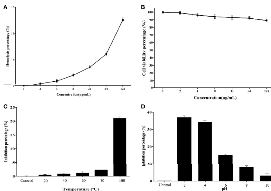
FIGURE 4 | Hemolytic effect, cytotoxic effect, and stability of Cc-AFP1. (A) Cc-AFP1 hemolytic effect against human erythrocytes. (B) Cytotoxic effect of Cc-AFP1 against HEK293 cells. (C, D) The temperature (C) and pH (D) effects on the antifungal effect of Cc-AFP1 against A. fumigatus cells. Values are provided as mean \pm SD.
