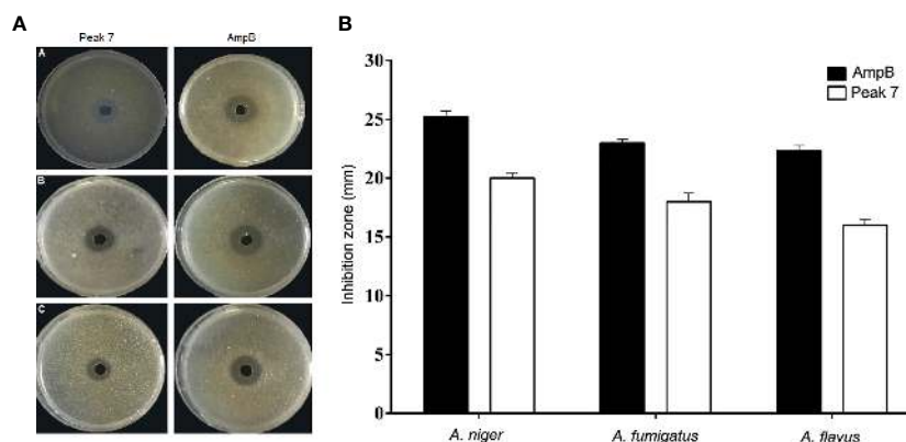
FIGURE 2 | (A, B) Antifungal effect of peak 7 against Aspergillus species was measured using the radial diffusion method. (A) The inhibition zone of peak 7 (2 \mu\text{g/well} ) and amphotericin B (0.2 \mu\text{g/well} ) against (A) A. flavus PFCC 50041, (B) A. niger ATCC 9142, and (C) A. fumigatus PFCC 50091. (B) Quantitative results of the inhibition zone diameters of peak 7 and AmpB for tested fungi with values that are given as the mean \pm SD.
