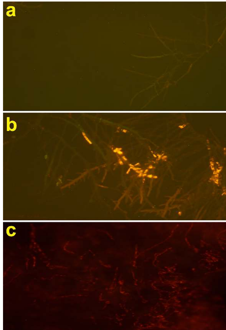
FIGURE 5 | Fluorescent microscope analysis of propidium iodide uptake during the membrane permeabilization assay. (A) Fluorescent images of untreated A. fumigatus hyphae. (B, C) Fluorescent images of treated A. fumigatus hyphae with Cc-AFP1 at the concentration of 8 and 16 µg/ml, respectively.
