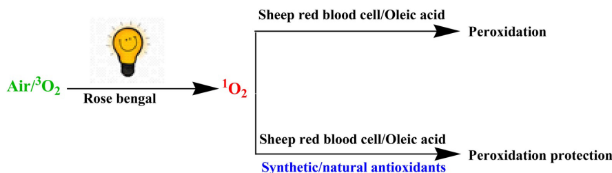
FIGURE 1 | Generation or quenching of ^1\text{O}_2 in red blood cells (erythrocyte) and oleic acid media in the presence and absence synthetic/natural antioxidants.
