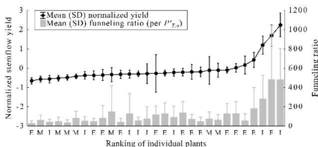
Figure 6. Mean and standard deviation (SD) of normalized stemflow yield per plant and the associated funneling ratio per Hertz (1986) and using modeled overstory throughfall ( P'_{T,o} ) in order of rank per mean normalized stemflow yield. Plant locations within clusters are indicated as follows: E denotes external; M denotes middle, between the interior and exterior; and I denotes interior.
