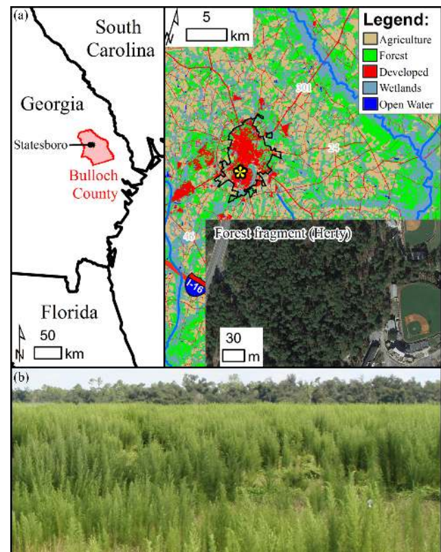
Figure 2. (a) Location of the studied Pinus palustris (longleaf pine) forest fragment, Charles H. Herty Pines Nature Preserve, on the Statesboro, Georgia (USA), campus of Georgia Southern University, where Eupatorium capillifolium (dogfennel) is a dominant understory plant. (b) Dogfennel can dominate pastures as well, as shown by the photograph (credit: Brent A. Sellers). The map layers were sourced from state and county boundaries and aerial imagery ©Esri, TomTom North America, Inc. The land use layer was derived from the National Land Cover Database 2011 (full metadata and data access link: https://gdg.sc.egov.usda.gov/Catalog/ProductDescription/NLCD.html , last access: 22 July 2019).
