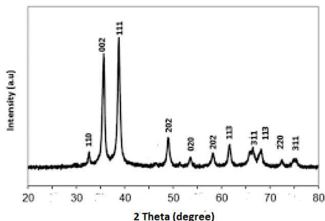
Fig. 2: XRD of synthesized copper oxide nanoparticles
