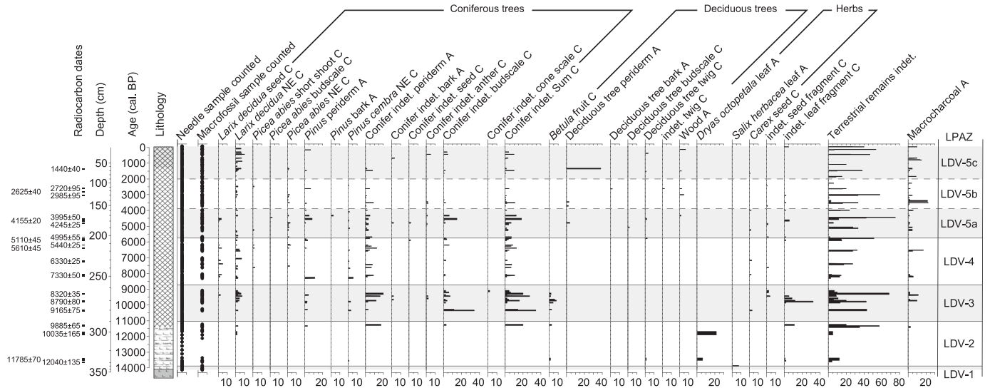
Fig. 4. Summary macrofossil diagram. Plant and macrocharcoal concentration per 20 cm^3 . Indet. = indeterminate, C = counts, A = area in mm^2 , NE = needle equivalent. LPAZ correspond to statistically significant local pollen assemblage zones 1–5.
