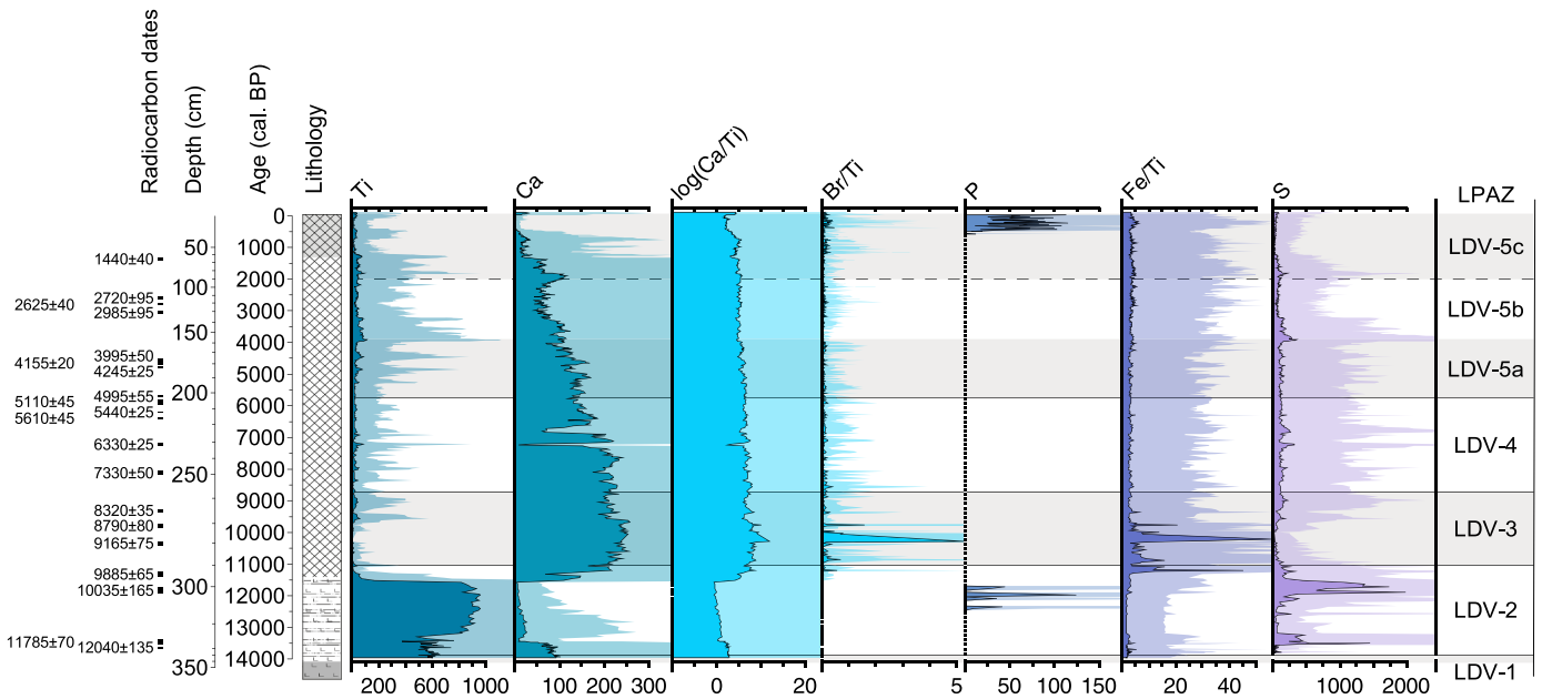
Fig. 3. XRF results of Lai da Vons (in counts s^{-1} , cps). Ti: Titanium (lithogenic input); Ca: Calcium (endogenous carbonate, lake water temperature, and productivity); log-transformed Ca/Ti ratio (endogenous carbonate, lake water temperature, and productivity); Br/Ti ratio: Bromine (organic material, productivity); P: Phosphorous (sedimentary P-retention); Fe/Ti ratio (authigenic iron); S: Sulfur (reducing conditions, authigenic sulfide formation). Lighter shades show a 10x exaggeration. LPAZ correspond to statistically significant local pollen assemblage zones 1–5.
