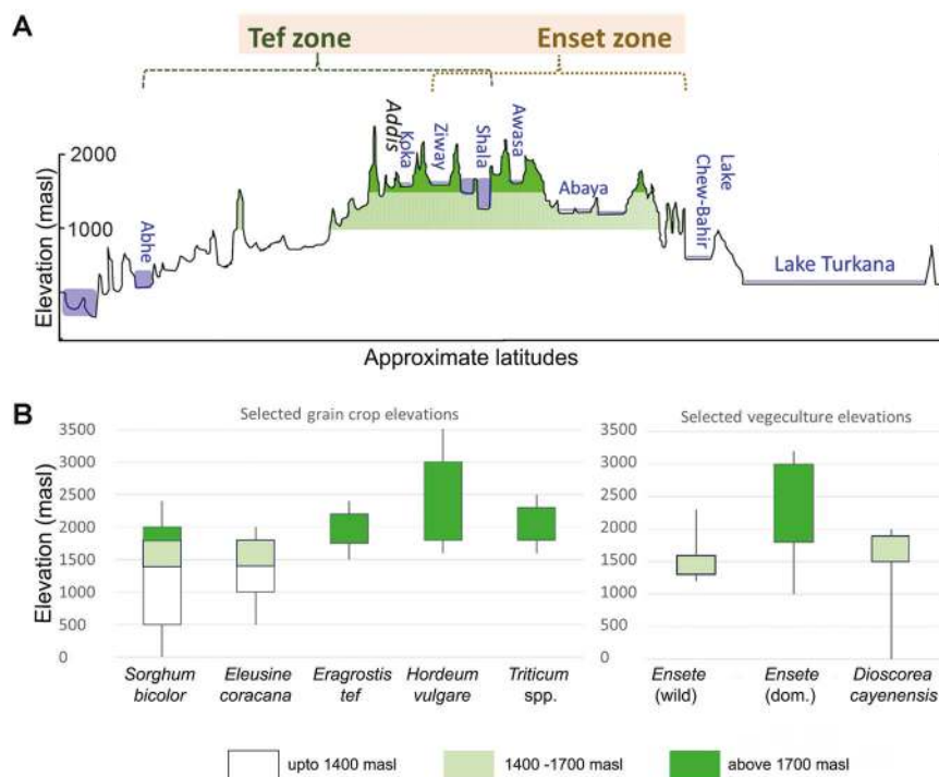
Figure 3. A: Diagram showing the elevational ranges in Ethiopia along a transect from north to south, and where tef and enset grow; lake basin names are indicated as is the approximate latitude of Addis Ababa (in italics). B: Box plots showing the elevation ranges for selected grain and vegetative crops cultivated in Ethiopia. Dark green indicates higher elevations where enset is a predominant crop (>1800 m asl), lighter shading indicates an intermediate zone of generally higher agrobiodiversity and less enset, and lower elevations (up to 1000 m asl) are not shaded.
