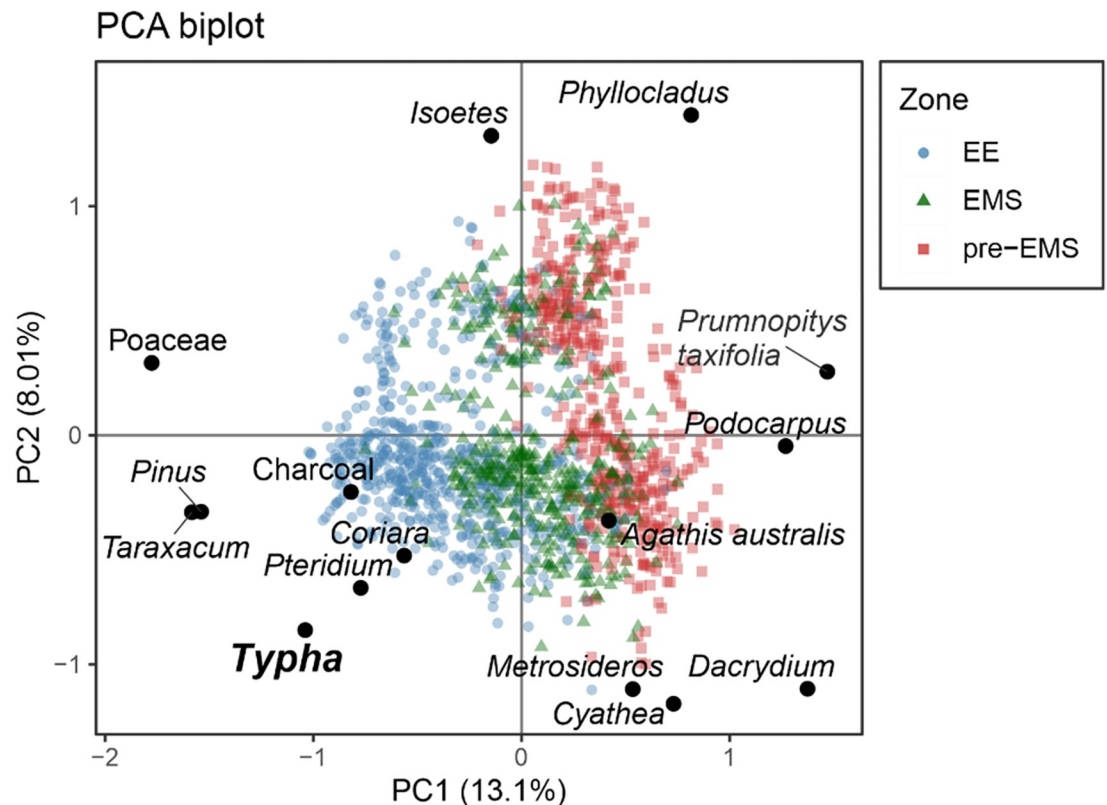
Fig 7. Biplot of taxa and sample scores on the first two principal component (PC) axes for 86 pollen records from lakes in Aotearoa New Zealand, spanning approximately the last millennium. The most common pollen taxa are labelled on the diagram. The same plot but with a more complete illustration of taxa scores is available in S1 Fig and S2 Table .
