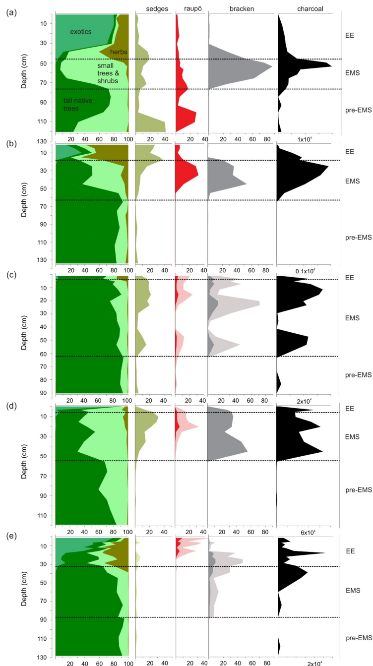
Fig 6. Raupō and cyperaceae pollen and Pteridium spore curves along with summary ecological groups at key pollen sites indicating different temporal patterns of raupō increase (see text for description of categories). Pollen and spore counts are percentages, charcoal counts are number of specimens per cm 3 of sediment sample. (a) Category I, Lake Kereta; (b) Category II a, Lake Kohangapiripiri; (c) Category II b, Lake Mangarakau; (d) Category II c, Lake Te Kahika; (e) Category III, Lake Killarney. See S1 Table for information on lakes including location.
