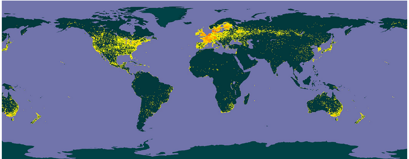
Fig 1. Global distribution of Typha spp. Source: Global Biodiversity Information Facility. Base map and data from OpenStreetMap and OpenStreetMap Foundation https://www.gbif.org/species/2702102 .
