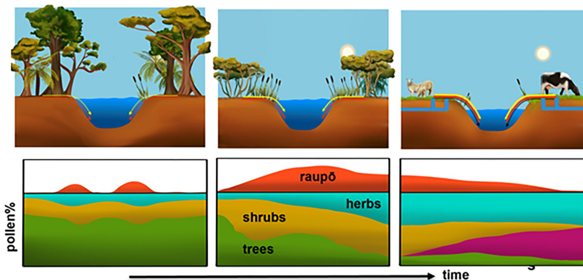
Fig 8. Schematic representation of raupō response to environmental changes during the last millennium in New Zealand (upper panels) informed by palynology represented as generalised pollen diagram (lower panels). In the upper panels arrows represent flux of nutrients (pink), sediments (vlu) and contaminants (black). Pre-EMS, EMS and EE phases as described in text.
