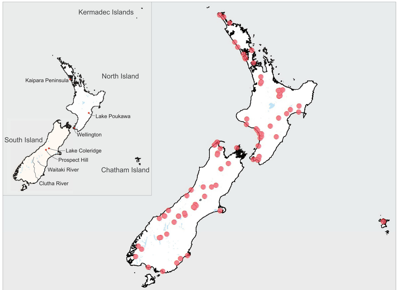
Fig 2. Aotearoa New Zealand showing location of sites mentioned in text (inset) and location of the lake sites investigated in this study as red dots (full map). Basemap showing Aotearoa New Zealand sourced from the LINZ Data Service and licensed for reuse under the CC BY 4.0 licence. ( https://www.linz.govt.nz/products-services/data/licensing-and-using-data/attributing-linz-data ).
