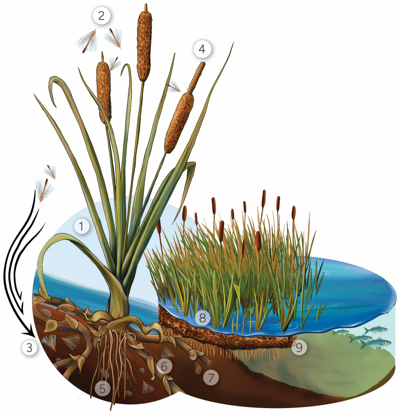
Fig 3. Schematic depictions of Typha individual (left) and community (right, reduced scale) illustrating various attributes promoting response to disturbance: 1. Large, resilient structures; 2. Small, wind-dispersed seeds; 3. Long seed-bank viability; 4. Flowers produce abundant pollen; 5. Aerated roots advantageous in organic-rich, flooded soils; 6. Rhizome carbohydrate storage maintains plant over winter and enables rapid spring growth; 7. Rhizomes anchor in substrate, trapping sediment and promoting lateral propagation; 8. Aggressive clonal propagation promotes dense monotypic stands; 9. Can spread across open water via floating rhizome mats.
