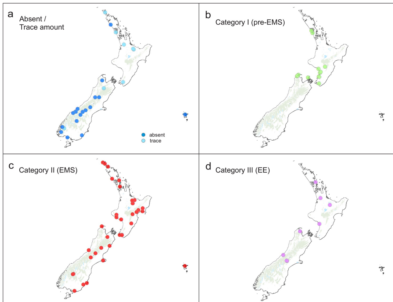
Fig 9. Spatio-temporal patterns of raupō from 92 pollen records from lakes in Aotearoa New Zealand during the past ~1000 years. Land elevation above 800 m a.s.l. shown in grey. (a) sites where raupō pollen is absent or in trace amounts; (b) category I where raupō expansion is observed pre-EMS; (c) category II where raupō expansion is first observed concomitant with or during Evidence for Māori Settlement (EMS); (d) where raupō expansion is first observed during the European era (EE). Basemap showing Aotearoa New Zealand sourced from the LINZ Data Service and licensed for reuse under the CC BY 4.0 licence. ( https://www.linz.govt.nz/products-services/data/licensing-and-using-data/attributing-linz-data ).
