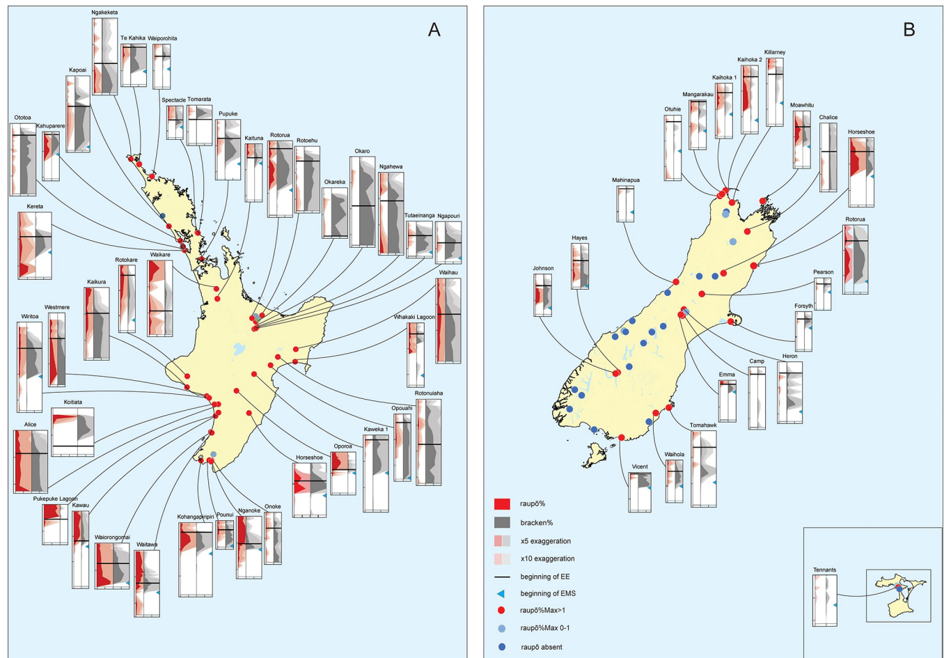
Fig 5. Reduced 2-taxa pollen diagrams showing raupō pollen and Pteridium spore percentages from lakes throughout Aotearoa New Zealand (A) Te Ika-a-Māui / North Island (B) Te Waipounamu / South Island. Inset: Chatham Islands. For each plot, Y axis is depth from surface of the lake bed in 50 cm increments and X axis increments are 25% for raupō and 50% for Pteridium . Blue triangles indicate earliest point after which sustained palynological evidence for human settlement occurred based on multiple palynological indicators including Pteridium (beginning of EMS). Areas in the maps coloured green represent aggregated clusters of archaeological sites based on https://nzarchaeology.org/archsite . A strong, albeit variable, stratigraphic association is illustrated between raupō and Pteridium —and hence with human settlement patterns—throughout both main islands, within its presumed natural limits. Basemap showing Aotearoa New Zealand sourced from the LINZ Data Service and licensed for reuse under the CC BY 4.0 licence. ( https://www.linz.govt.nz/products-services/data/licensing-and-using-data/attribution-linz-data ).
