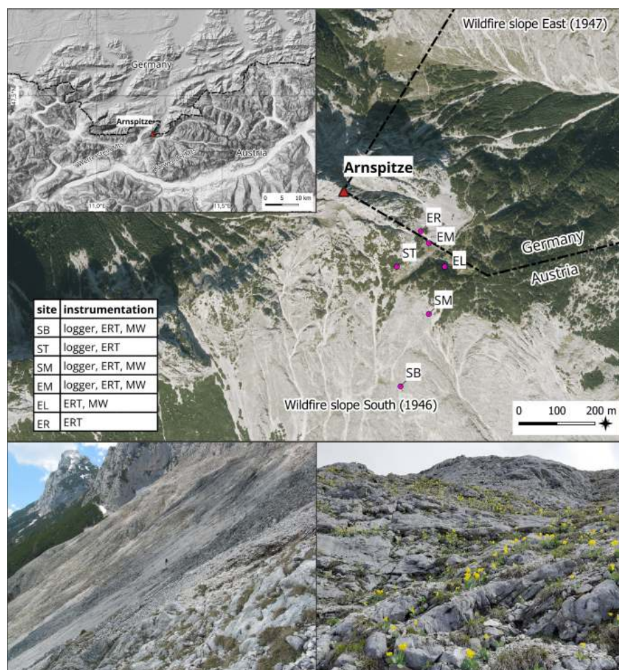
Figure 1. Location of the study area at the border between Germany and Austria (top left) and the study sites on the slopes of the Arnspitze; Background: OpenStreetMap (top left); hillshade and contourlines processed from digital terrain model of the state of Tyrol ( https://data.tirol.gv.at , last access: 2 December 2024). Photos from the south-facing slope by OS.
