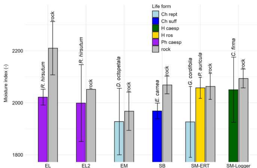
Figure 10. Dimensionless MW moisture index with cover of different plant species; 0–25 cm rock depth (life forms see Fig. 9).
