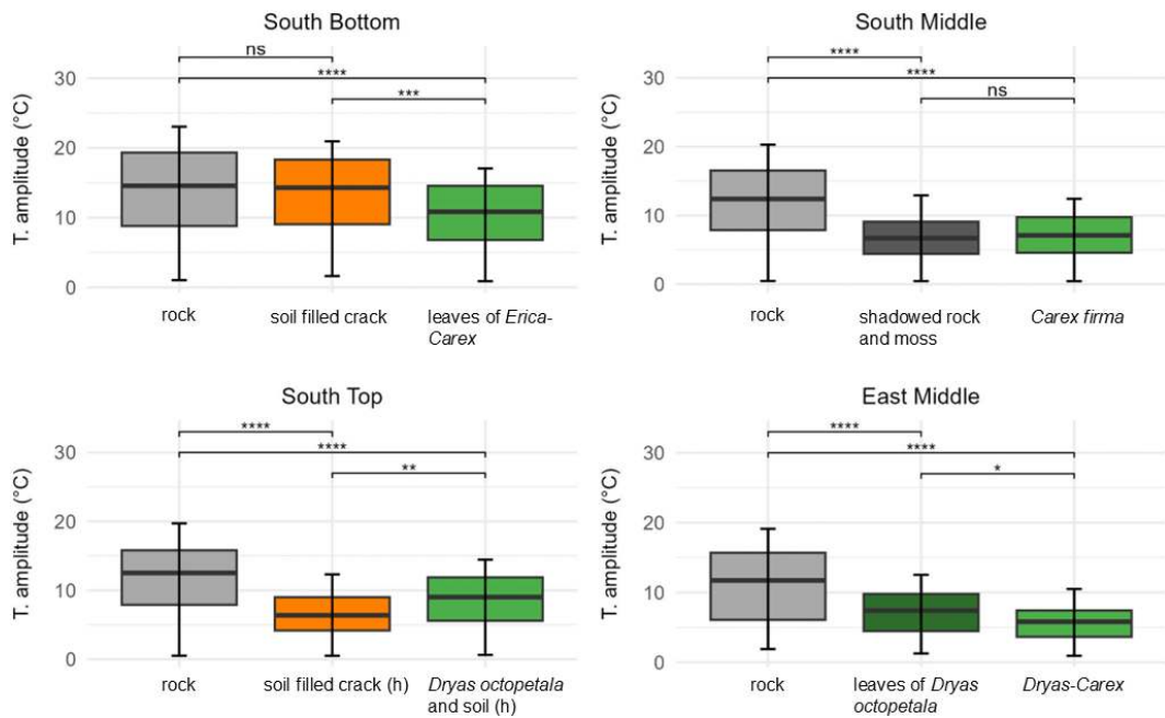
Figure 3. Distribution of the daily temperature amplitude in the rock with different cover at the surface from 27 May to 27 August (significance levels indicated by ns = not significant ( p>0.05 ), * p\leq 0.05 , ** p\leq 0.01 , *** p\leq 0.001 , **** p\leq 0.0001 ).
