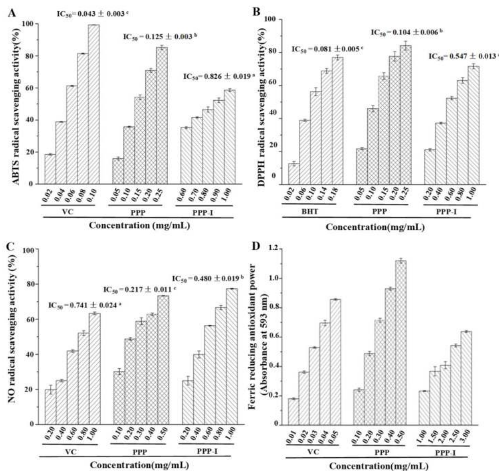
Figure 3. Stability of ABTS (A), DPPH (B), NO (C), and FRAP (D) antioxidant capacities of PPP after in vitro digestion. PPP, polyphenolic-protein-polysaccharide ternary complexes from Hovenia dulcis ; PPP-I, indicated PPP after in vitro digestion. BHT, butylated hydroxytoluene; VC, vitamin C. The error bars are standard deviations; Different superscript lowercase letters (a–c) indicated significance ( p < 0.05 ). Statistical significances ( p < 0.05 ) were carried out by one-way analysis of variance (ANOVA) followed by a Duncan's test.
