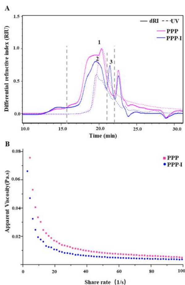
Figure 1. Changes in HPSEC chromatogram (A) and apparent viscosity (B) of PPP after in vitro digestion. PPP, polyphenolic-protein-polysaccharide ternary complexes from Hovenia dulcis ; PPP-I, indicated PPP after in vitro digestion.
