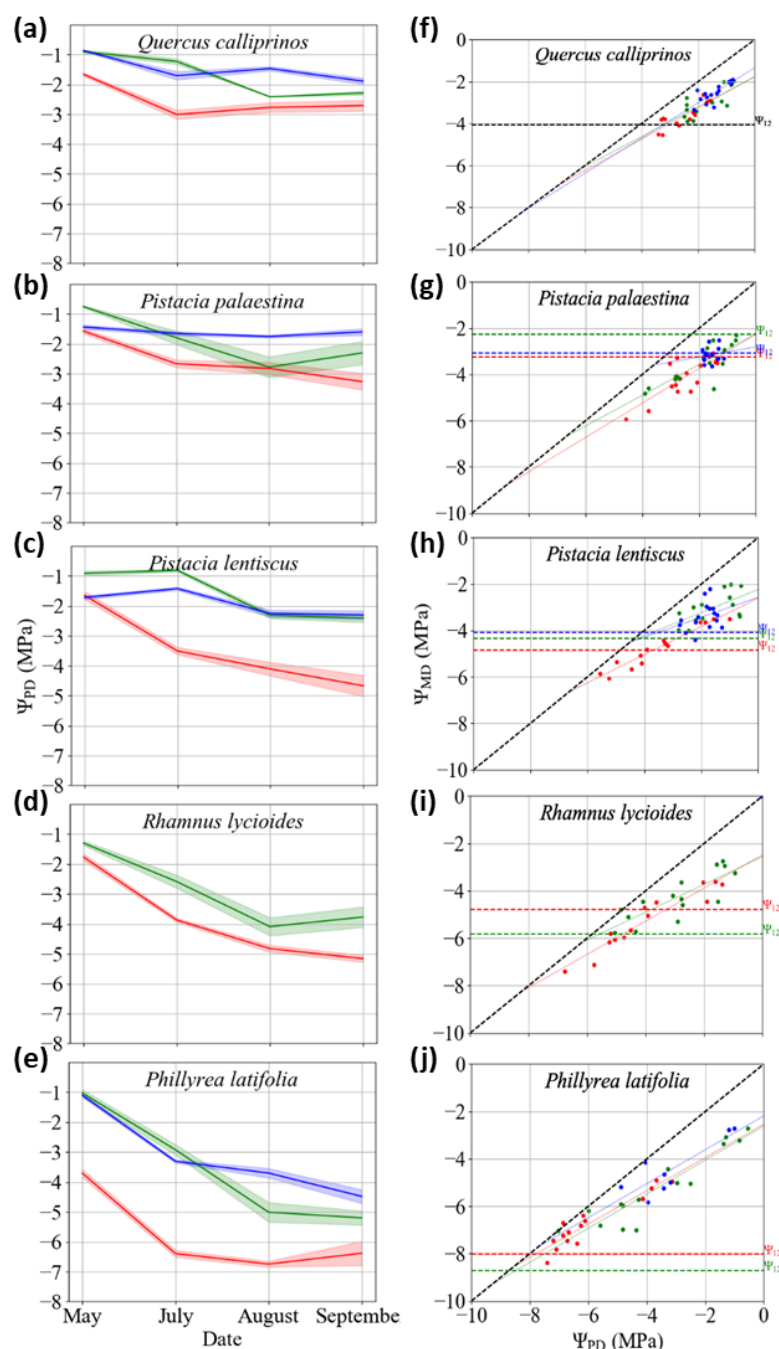
878 Fig. 3: Leaf water potential values during the dry season of 2018 at the Mesic- 879 Mediterranean (blue), Mediterranean (green), and Semi-arid (red) study sites. a-e; 880 Courses of predawn leaf water potential for each species. Line shadow represents 881 standard error. f-j, Midday water potential ( \Psi_{MD} ) vs. predawn water potential ( \Psi_{PD} ) 882 for all species during the dry season. Each point on a plot is the average of two twigs. 883 Regression parameters can be found in Table S3. Thick dashed black line represents 884 1:1 ratio. The thin colored lines are the regressions of all points of each site. Vertical 885 dashed lines indicate the point of incipient embolism ( \Psi_{12} ) values for the MM (blue), 886 M (green), and SA (red) sites. Vertical dashed black line in f indicate point of 887 incipient embolism based on Q. coccifera data (see Material and Methods section).
