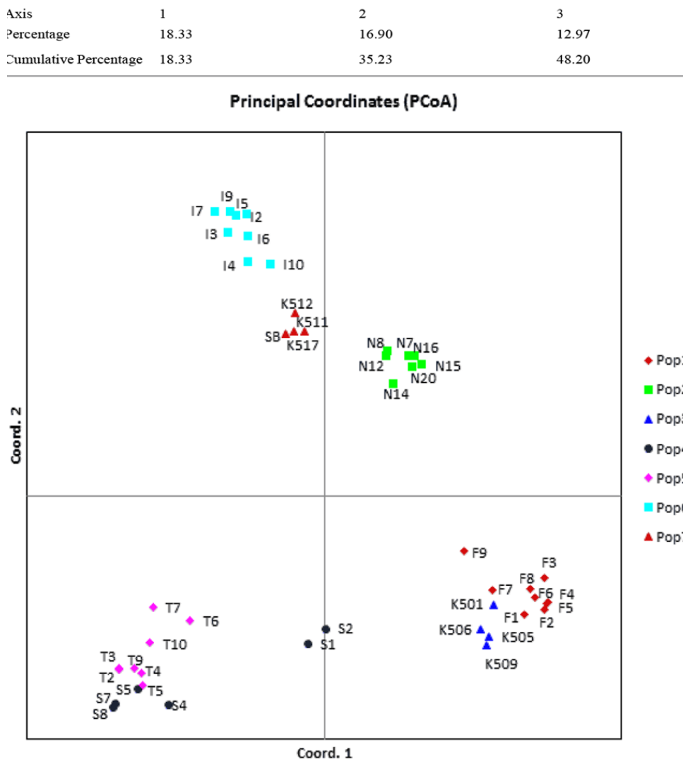
Figure 3. Two-dimensional scatter plot of PCoA axis generated for 42 Swertia chirayita accessions by 27 ISSR-PCR primers through Principal Co-ordinate Analysis.
