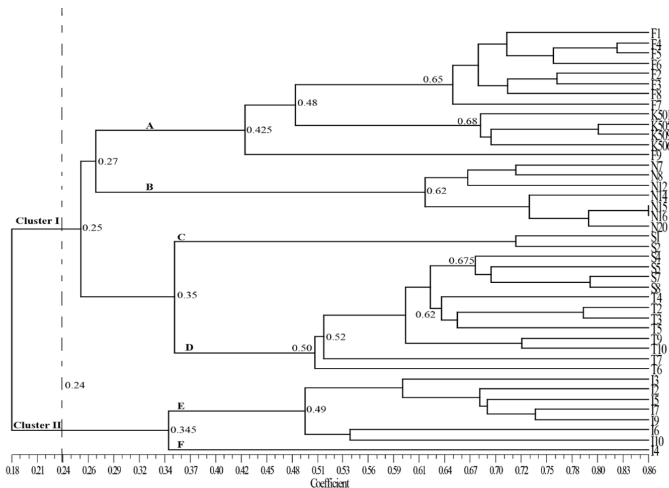
Figure 2. Dendrogram generated for 27 polymorphic ISSR-PCR primers data of 42 Swertia chirayita accessions using Jaccard's similarity coefficient by UPGMA method of Cluster analysis. The clusters are labeled as A, B, C, D.
