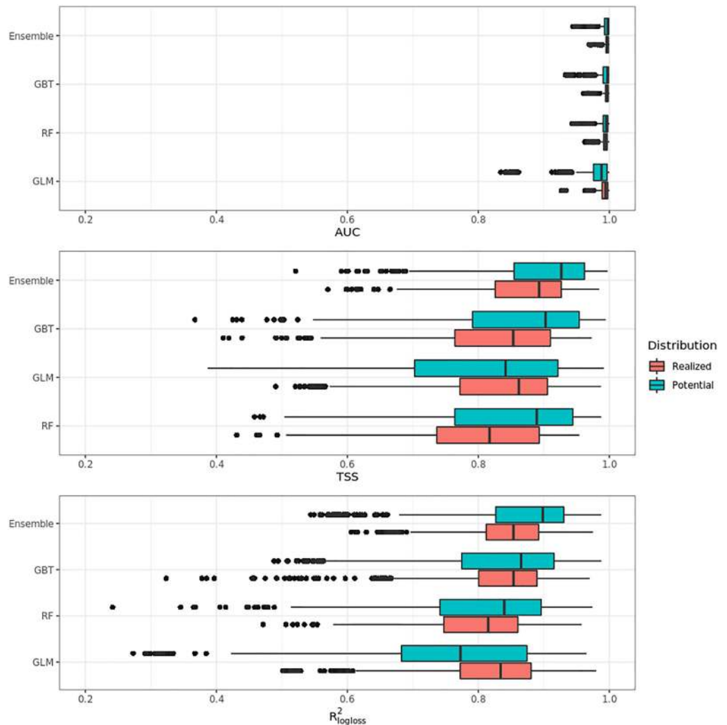
Figure 4 Aggregated results of the accuracy assessment per model and distribution expressed using AUC, TSS and R^2_{\logloss} .
