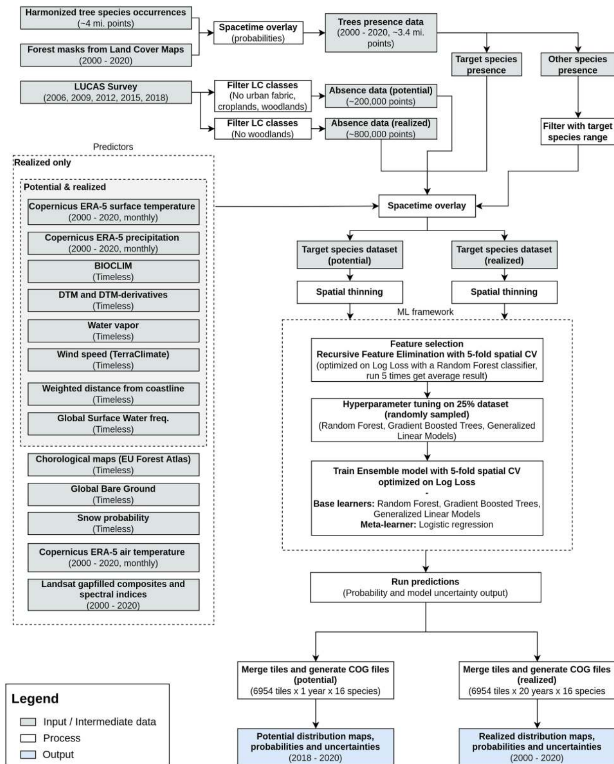
Figure 1 General workflow illustrating the preparation of the point data, the predictor variables used, model building (feature selection—hyperparameter optimization—training) and preparation of distribution maps for one species. The process was identically replicated for all the species. Full-size DOI: 10.7717/peerj.13728/fig-1
