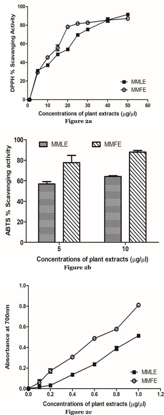
Figure 2. Antioxidant capacity of MMLE and MMFE. (a) DPPH % scavenging activity of MMLE and MMFE at different concentrations (1.0 – 50.0 µg/µl). (b) Dose-dependent ABTS % scavenging activity of MMLE and MMFE (5.0 µg/µl and 10.0 µg/µl). (c) Free radical scavenging activity of MMLE and MMFE as calculated by reducing power assay at various concentrations (0.1 – 1.0 µg/µl).
