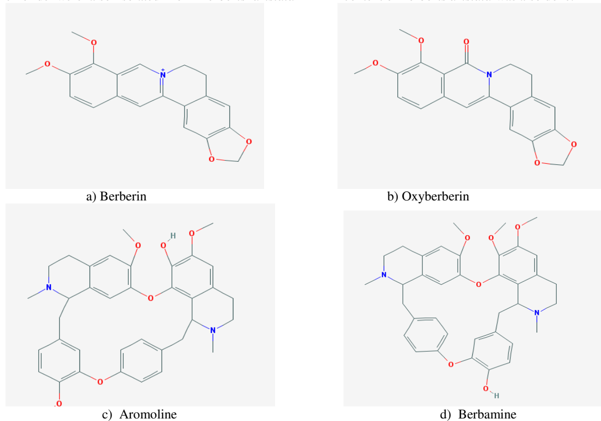
Figure 3: Structure a) Berberin, b) Oxyberberin, c) Aromoline, d) Berbamine
