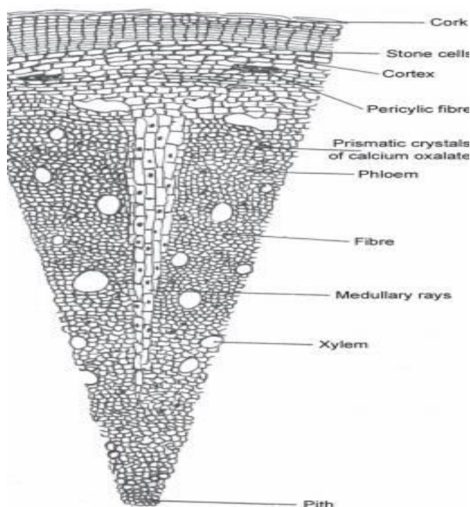
Figure 2: T.S. of Berberis aristata DC stem
