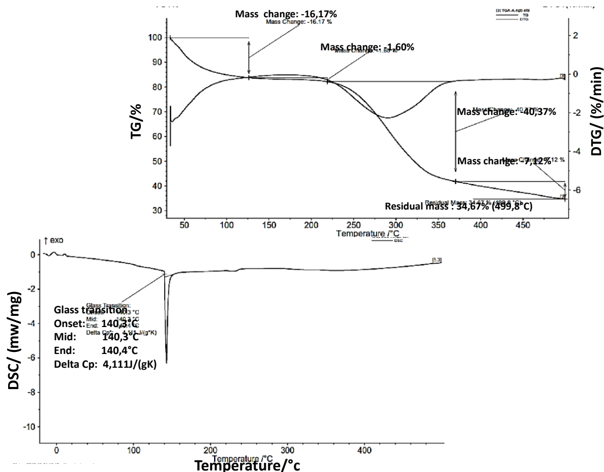
Figure 9. Differential Scanning Calorimetry graph of Grewia spp. biopolymer
